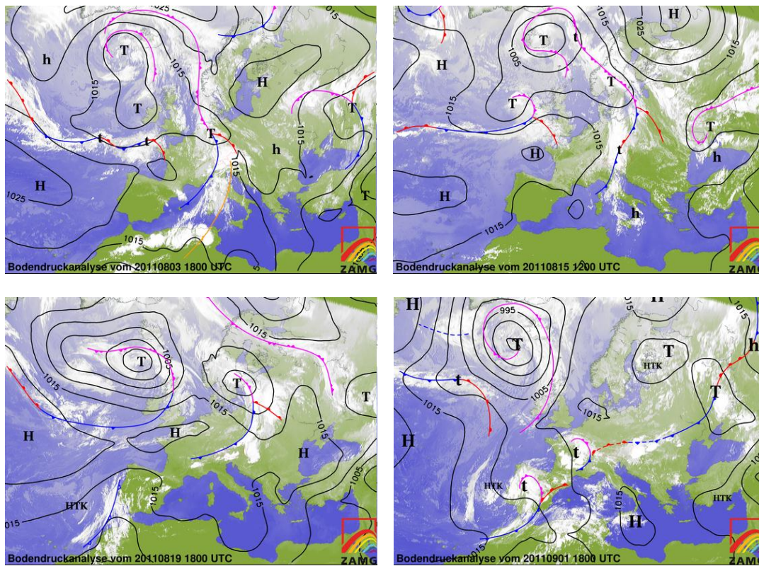
Figure 5. Satellite image, surface pressure analysis and frontal zones on the four selected days. Top left: 03 August 2011, 18:00 UTC; top right: 15 August 2011, 12:00 UTC; bottom left: 19 August 2011, 18:00 UTC; bottom right: 01 September 2011, 18:00 UTC.
