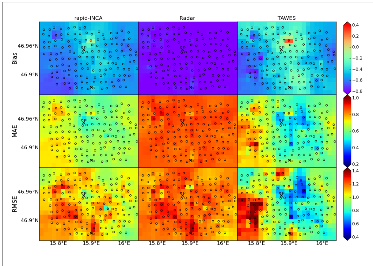
Figure 12. Relative bias, MAE, and RMSE for rapid-INCA, radar and TAWES stations at each WegenerNet station. Only those data points are included where the WegenerNet station measured more than 0.5 mm/5 min. Circles represent exact values at the WegenerNet stations, the image is obtained by IDW interpolation to the INCA grid
