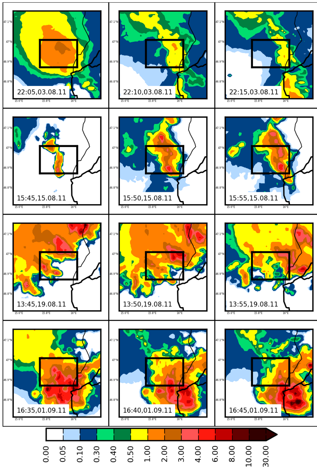
1 2 Figure 6. Spatio-temporal distribution of rapid-INCA precipitation (mm/5min) in the region 3 of the WegenerNet indicated by the black rectangle (time is given in UTC).
