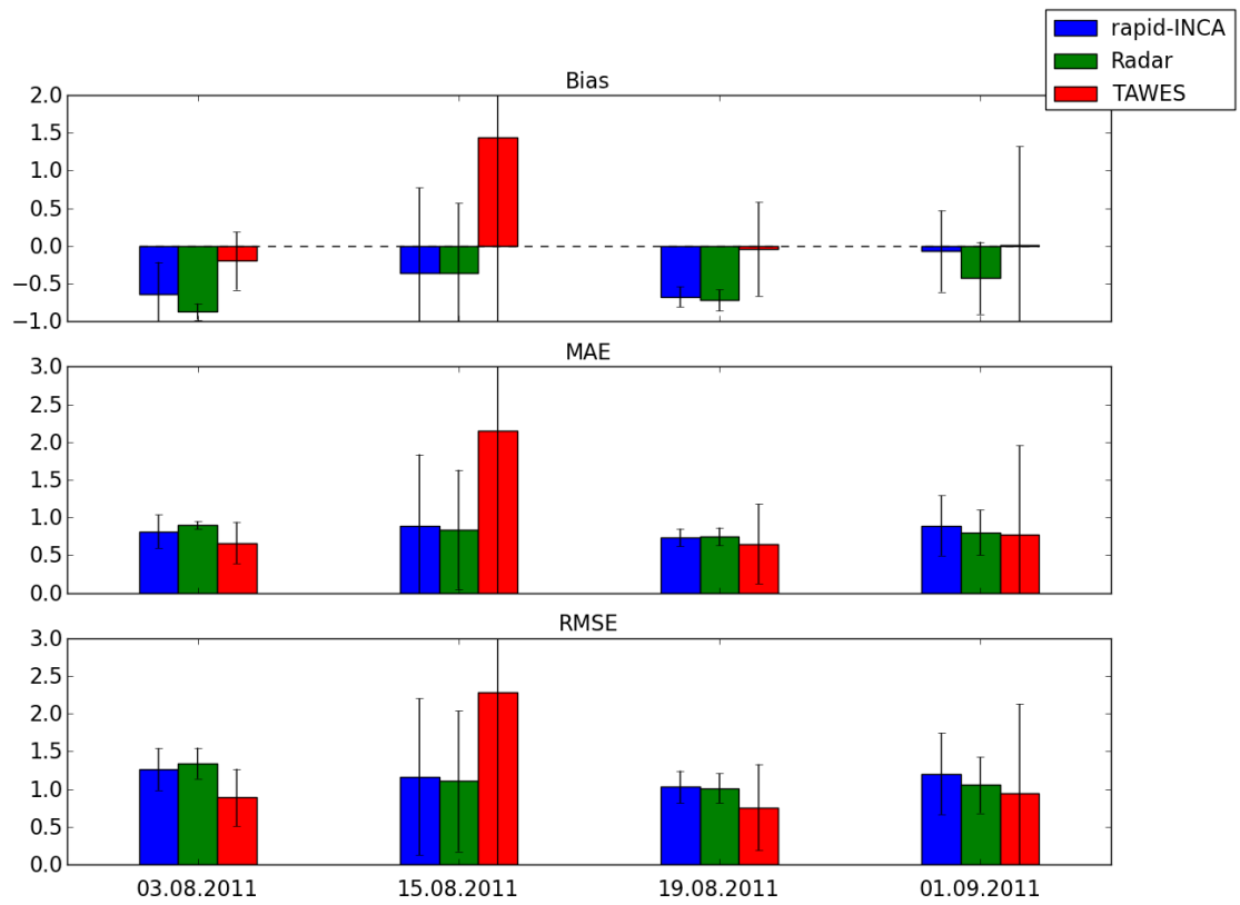
Figure 8. Relative bias, MAE, and RMSE (weighted by the mean observed precipitation of WegenerNet). Values have been computed for each of the WegenerNet stations (151 stations) and then averaged over space. Error bars represent the standard deviation of obtained verification measures at each WegenerNet station.
