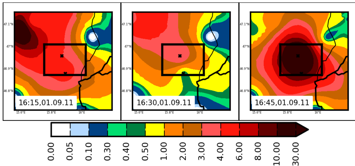
Figure 9. Spatio-temporal distribution of 15-minute interpolated TAWES station measurements (mm/15min) on 01.09.2011 between 16:15 and 16:45 UTC (region of WegenerNet is shown by the black rectangle and the two TAWES stations of ZAMG are marked with a cross).
