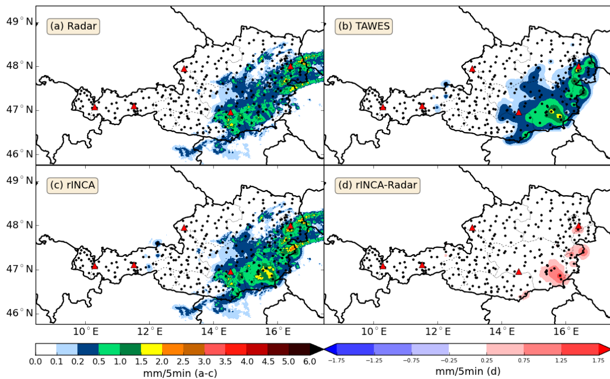
Figure 3. Example of a 5-minute precipitation analysis (rapid-INCA) based on the combination of rain gauge data and radar derived QPE on 13 September 2014, 02:40 UTC. (a) scaled radar field, (b) interpolated rain gauge measurements (TAWES), (c) final rapid-INCA precipitation analysis and (d) difference between rapid-INCA and radar derived QPE.
