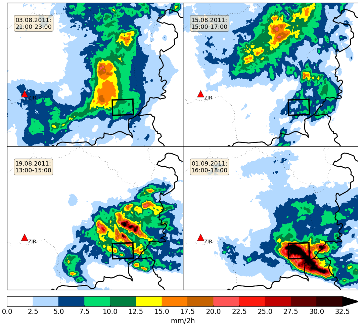
Figure 4. 2-hour precipitation accumulations of the 5-minute rapid-INCA analyses on four days (top left: 03 August 2011, top right: 15 August 2011, bottom left: 19 August 2011, bottom right: 01 September 2011) in the respective time spans. The WegenerNet region is marked by a small black rectangle, the red triangle represents the radar (Zirbitzkogel) within this zoom.
