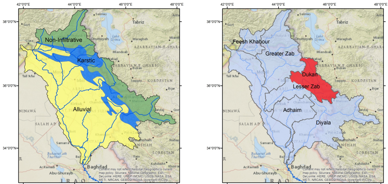
Figure 4. (left) Approximate division of Northern Iraq into three geologic zones, mainly based on (Stevanovic and Iurkiewicz, 2008). (right) Boundaries of main tributaries of the Tigris in Northern Iraq. The Dukan catchment, which is the upper part of the Lesser Zab catchment, is indicated in red. Calibration on streamflow is based on measurements from the Dukan area and calculation of water mass for the whole of Northern Iraq is based on all catchments.
