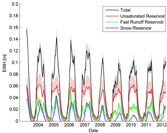
Figure 11. Water mass of the snow, unsaturated and fast runoff reservoir smoothed over 10 days. Lines represent optimal model and the bandwidth the Pareto ensemble based on NS and logNS of streamflow.
