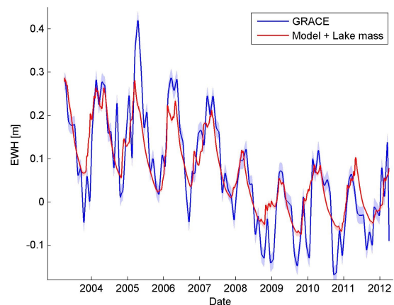
Figure 12. Comparison between resulting mass variation from GRACE and mass variation from lakes and rainfall-runoff model.
