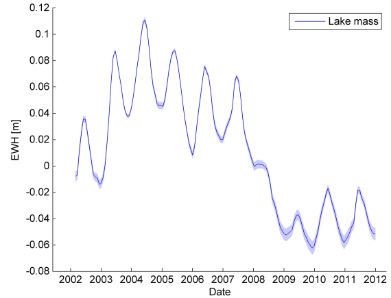
Figure 8. Lake mass variation.
