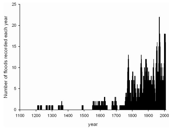
Figure 3. Number of floods with a recorded/estimated discharge exceeding the 0.8 threshold.
