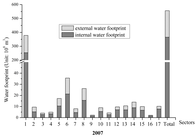
Fig. 3. Figure 2b. WFs in the HRB in 2007
