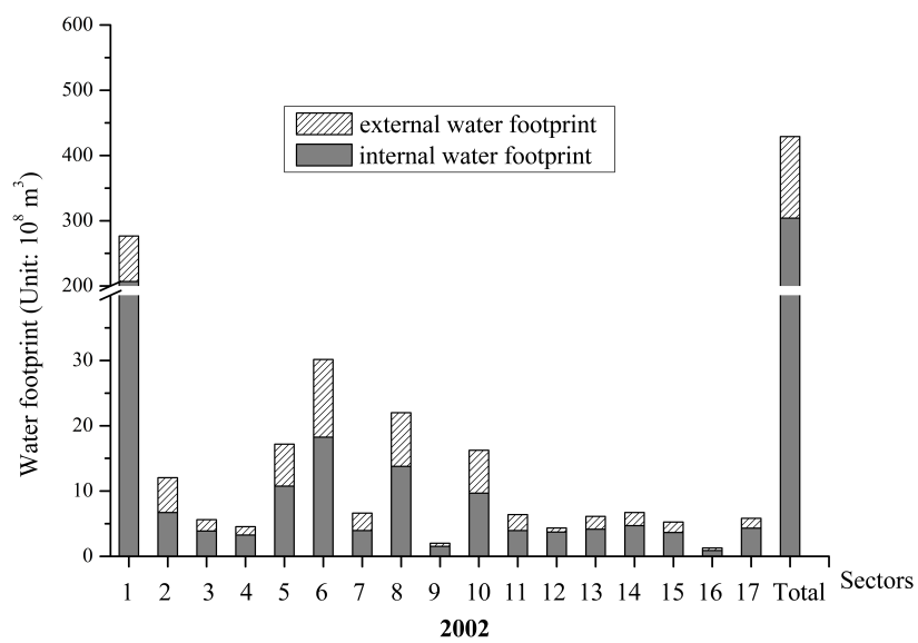
Fig. 2. Figure 2a. WFs in the HRB in 2002
