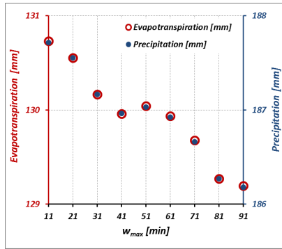
Fig. 3: Estimated sum of evapotranspiration and precipitation for the time from January 1 st , 2010 to May 2 nd , 2010 with varied filter parameter w_{max} .
