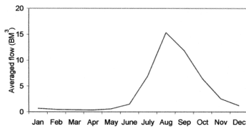
FIG. 1. Mean monthly flows for the Blue Nile River at Eldeim for the period 1913–89.
