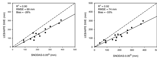
Fig. 11. Scatterplots of monthly SWE (at the 39 SNOTEL sites) from the SNODAS and the (A) SWE from the DisUEB with MPE precipitation and the original GFS's air temperature for January 2006–April 2008, and (B) SWE from the DisUEB with MPE precipitation and the original GFS's air temperature increased by 2 degree Celsius.
