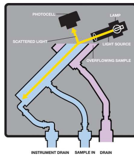
Schematic illustration of the turbidimeter.
