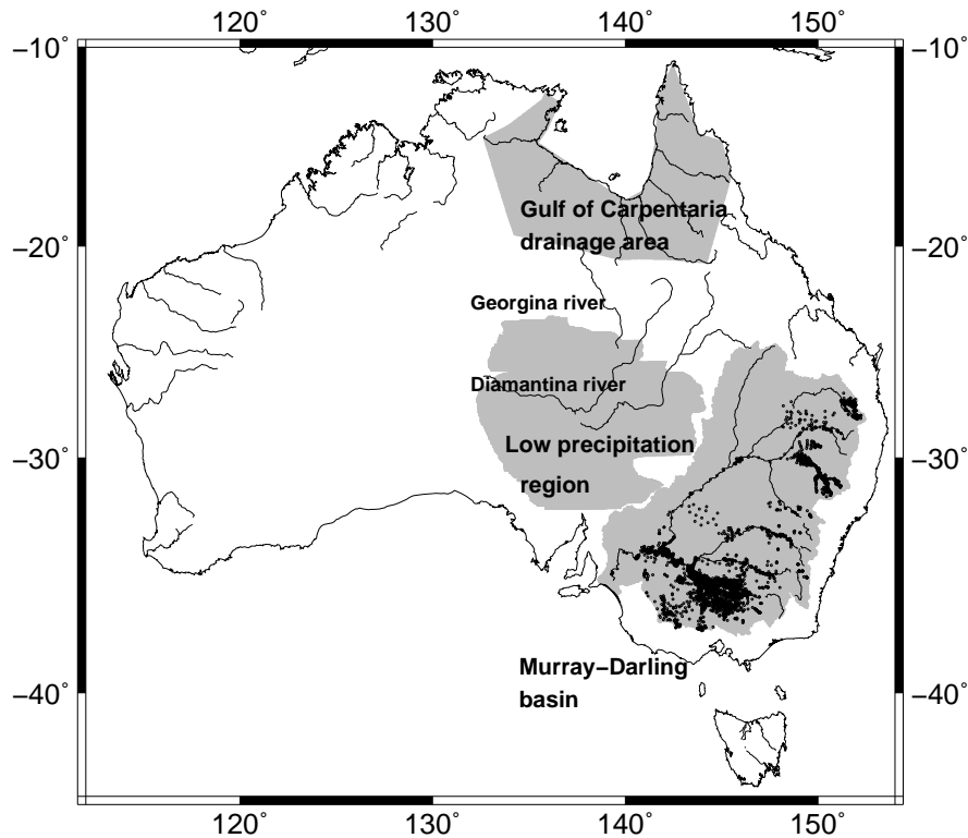
Fig. 1. Australian drainage regions used in our study. Geographical locations of the bores in the Murray–Darling are marked as black circles.
