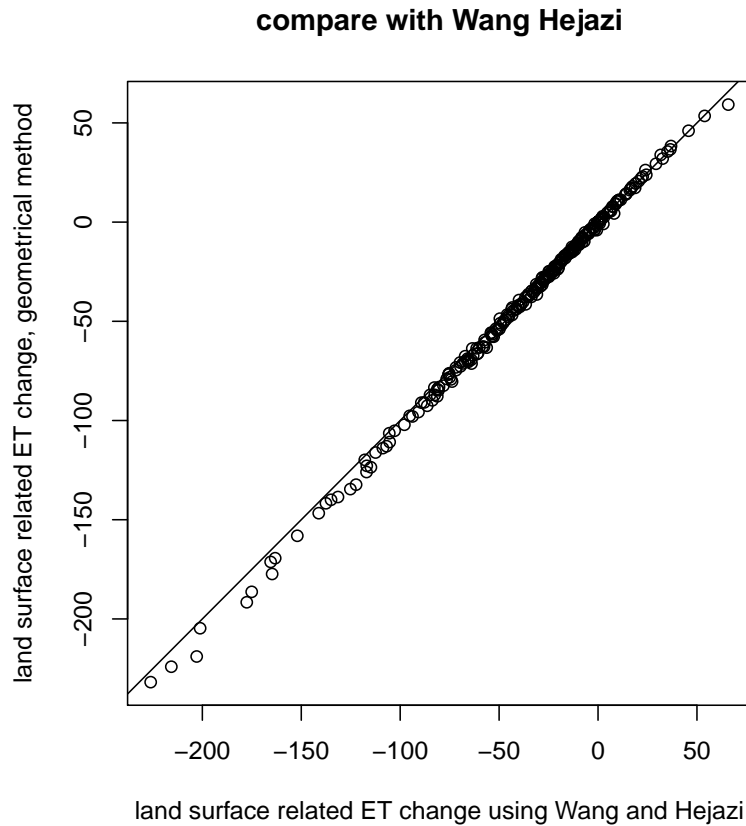
Fig. 4. Comparison of the estimated land surface change impact with the method of Wang and Hejazi (2011) for all basins in mm/yr.
