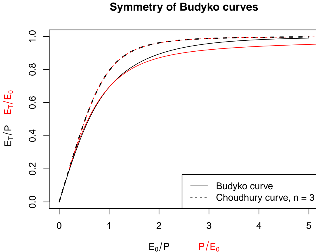
Fig. 3. Budyko space plot of the Budyko (lines) and Choudhury curves (dashed) for both, E_T/P vs. E_0/P (black) and E_T/E_0 vs. P/E_0 (red).
