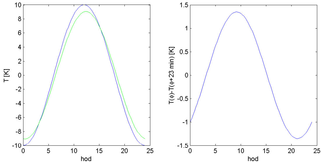
Fig. 1. Simulation of effect of phase difference on DTC.
