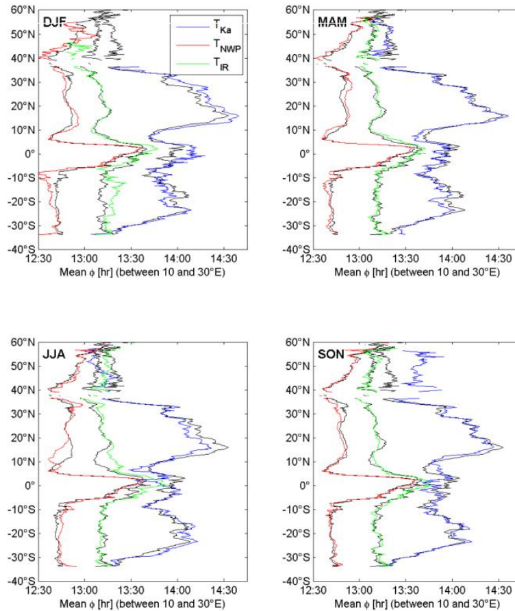
Fig. 2. North south transects of average phi, repeated for 3-month periods.
