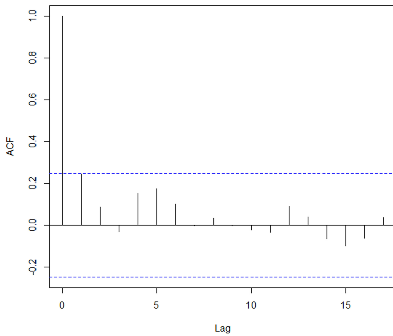
Fig. 4. Autocorrelation function: Bra 12h
