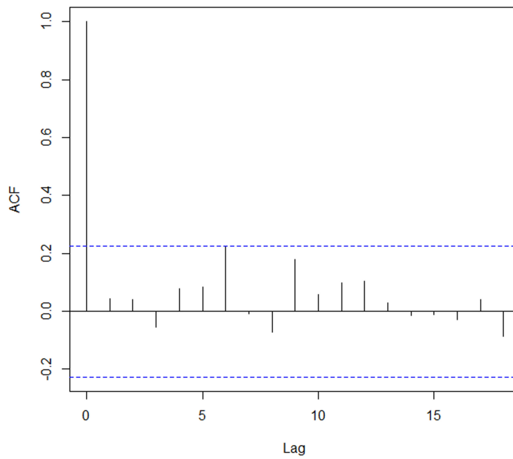
Fig. 2. Autocorrelation function: Bra 3h
