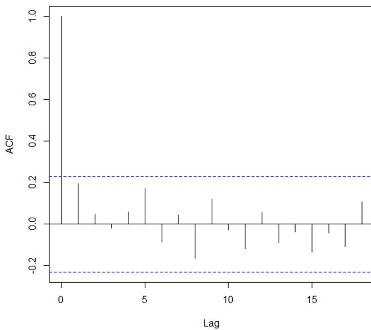
Fig. 3. Autocorrelation function: Bra 6h
