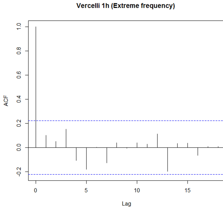
Fig. 5. Autocorrelation function: Vercelli 1h
