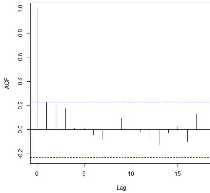
Fig. 1. Autocorrelation function: Bra 12h
