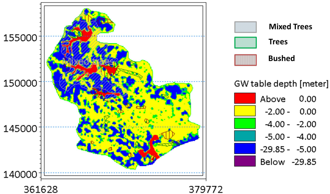
Fig. 2. Groundwater (GW) table depth and vegetation distribution Marina-like catchment
