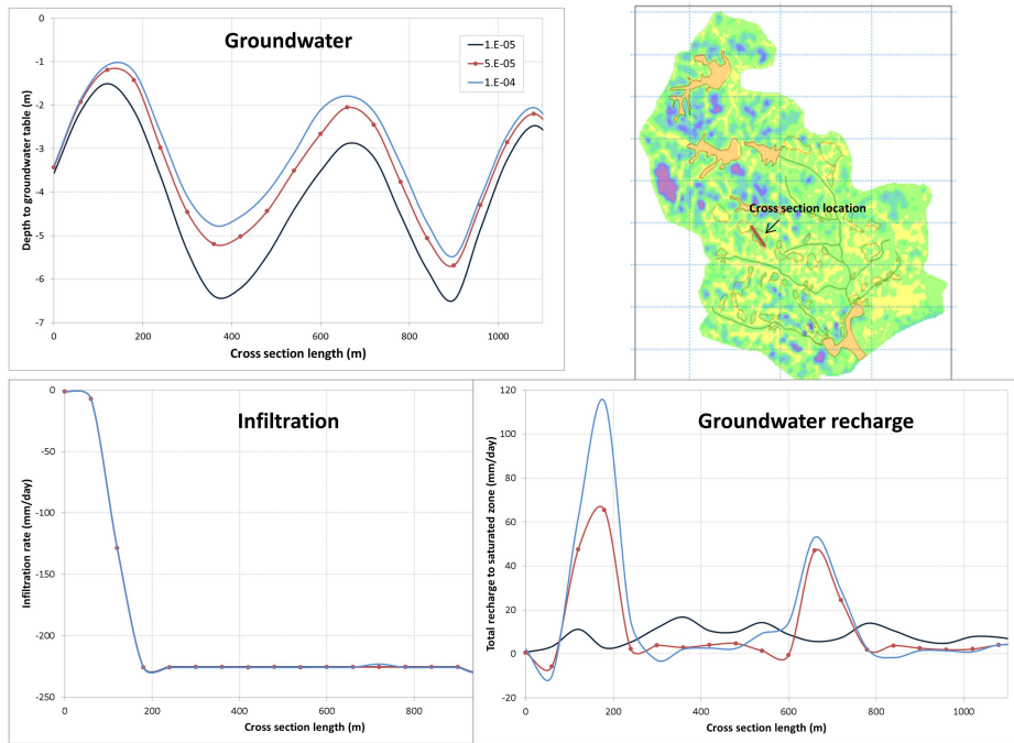
Fig. 1. Groundwater depth, infiltration rate and groundwater recharge across bio-retention systems with different soil hydraulic conductivity. Results are from 12 hours after largest rainfall event (130mm)
