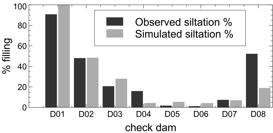
Fig. 1. Sediment sub-model spatial validation.
