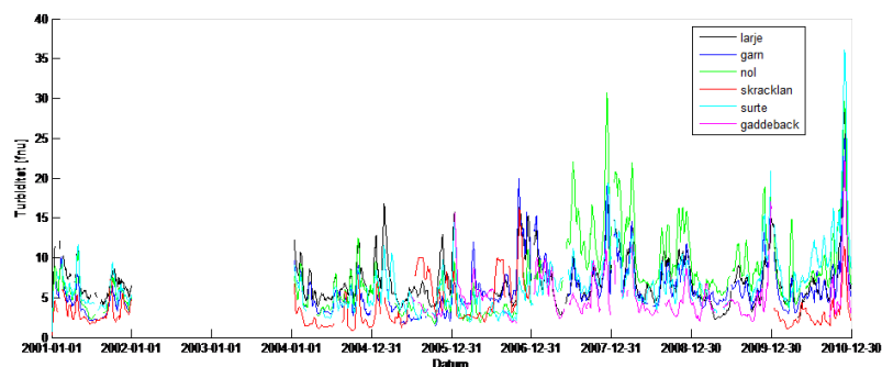
Fig. 1. 1. Measured turbidity at the gauging stations, 2001-2010
