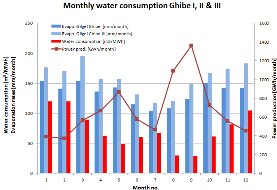
Fig. 3. The graph presents the monthly evaporation rates from the two reservoirs supplying Ghibe I, II and III power plants with water, monthly power production from the year 2005 and correspondingly monthly (gross) water consumption estimates (based on Yesuf, 2012).
