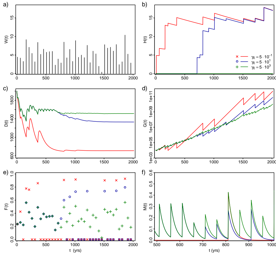
Fig. 4. The evolution of WetTown assuming a slow decay of protection levels (i.e. \kappa_T = 3 \times 10^{-4} \text{ yr}^{-1} ): (a) high water levels [m]; (b) flood protection levels [m]; (c) distance of WetTown from WildWaters River [m]; (d) size/wealth of WetTown [m 2 ]; (e) relative flood damages [.]; (f) awareness of the risk of flooding [.]. The colour of lines and points refers to the three scenarios: low-cost (red), moderate-cost (blue) and high-cost (green).
