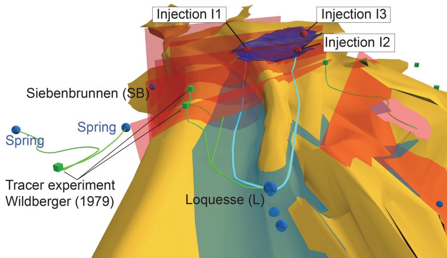
Fig. 3. 3-D view towards the East of the Urganian limestone basis (top of Valanginian Marls). Red and transparent planes are faults. Tracing experiments previously carried out are represented in green, including the expected underground flow paths. The Plaine Morte is visible in the middle (dark blue). Blue spheres are karstic springs. The blue surfaces with some transparency are karstic nappes.
