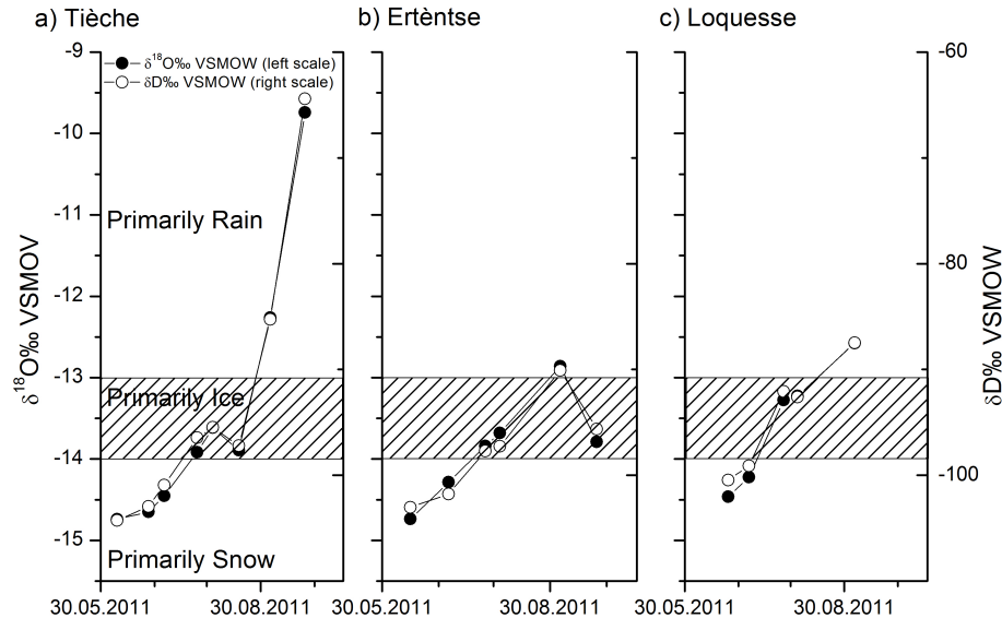
Fig. 8. Temporal development of isotopic composition at selected karst springs south of the Plaine Morte. Typical isotopic signatures found in snow samples are illustrated with striped area. Locations are shown in Fig. 1.
