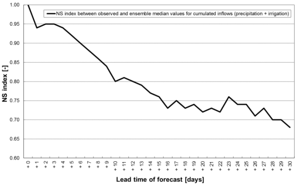
Fig. 4: The NS index for rainfall and irrigation amounts between the observed data and the median of 20 ensembles of the REPS-WRF model for the 2012 growing season over a period of more lead time days.
