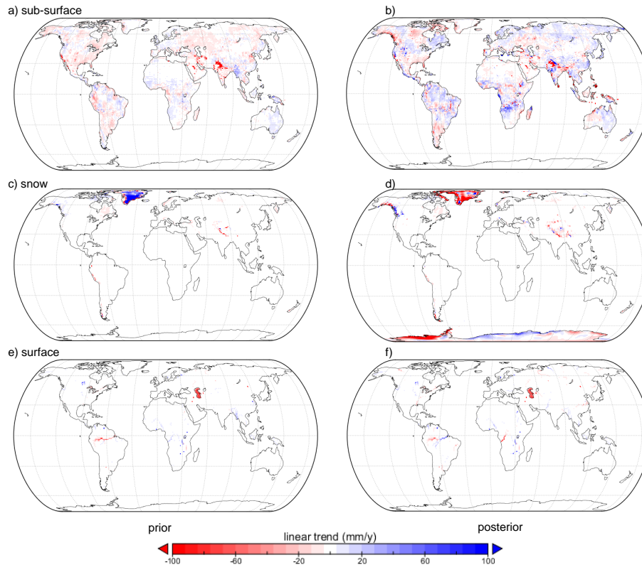
Fig. 5. Trends in seasonal anomalies of prior (left column) and posterior (right column) estimates of (a–b) sub-surface, (c–d) snow and (e–f) surface water (i.e., lake and river) water storage.
