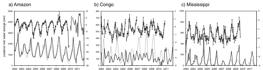
Fig. 8. Effect of assimilation agreement with satellite altimetry river water levels for grid cells including the (a) Amazon River ( \sim 2.5^\circ S, 65.5^\circ W; \rho changed from 0.71 for prior to 0.80 for posterior estimates); (b) Congo River ( \sim 2.5^\circ N, 21.5^\circ E; \rho from 0.28 to 0.47) and Mississippi River ( 35.5^\circ , 90.5^\circ W; \rho from 0.37 to 0.56).
