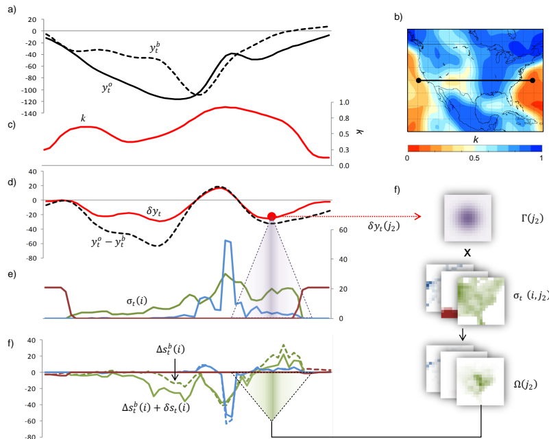
Fig. 1. Illustration of the data assimilation approach followed using data along a transect through the USA for August 2003. Shown are: (a) monthly satellite-derived TWS, y_t^o , and the equivalent prior estimate, y_t^b ; (b) location of the transect on a map of the gain matrix, k ; (c) profile of k along the transect (cf. Fig. 2c); (d) calculation of the TWS analysis increment, \delta y_t , from k and innovation, (y_t^o - y_t^b) ; (e) the prior error in the change of each of the stores, \sigma_t^b(i) and \sigma_t^b(i) + \delta s_t(i) , resp.; and (f) visual illustration of the disaggregation of the TWS analysis increments to the different stores. All units are in mm unless indicated otherwise; see text for full explanation of symbols; stores shown include the sub-surface (green), rivers (blue) and sea (dark red; remaining stores not shown for clarity).
