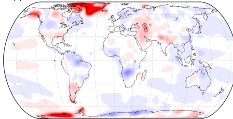
Fig. 4. Trends in GRACE total water storage as derived from (a) prior storage estimates; (b) merged satellite retrievals; and (c) posterior estimates.
