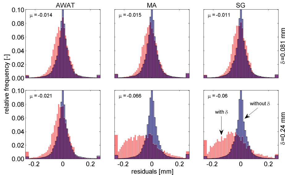
Fig. 8. Relative residual frequency distribution for the complete data set and the different filters with w = w_{\max} = 31 min. Blue bars indicate residuals between original and filtered data for the cases with mere smoothing, omitting the threshold values; red bars indicate cases with threshold values of either 0.081 (top panels) or 0.24 mm (bottom panels). The broad bars at plot edges comprise all residuals greater than 0.25 or smaller than -0.25 mm.
