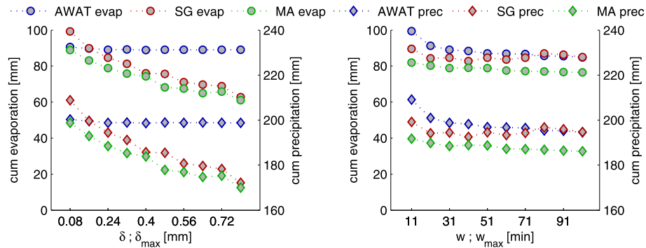
Fig. 10. Estimated sum of evaporation and precipitation for the time from 5 July to 7 October 2012. Left panel: varied filter parameter: \delta or \delta_{\max} . Right panel: varied filter parameter: w or w_{\max} .
