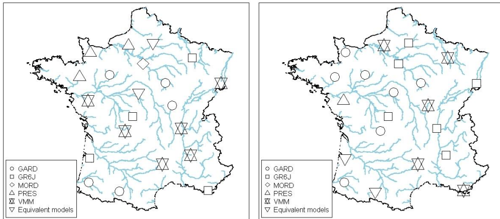
Figure 16: Maps of the model best ranked in forecasting for the mean of all criteria and for validation periods 1 (left) and 2 (right), for a d+7 forecasting lead time.
