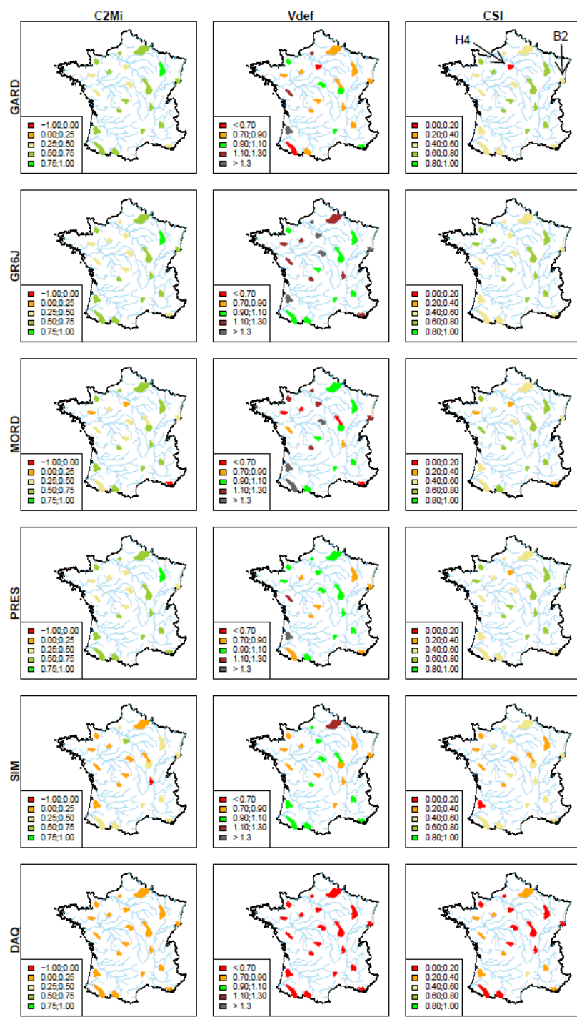
Figure 5: Maps of mean performance on the two validation periods in-for the C2Mi, Vdef and CSI criteria, obtained by for the five tested models tested and the benchmark (DAQ) on the 21 catchments, in simulation mode . The letters on the
