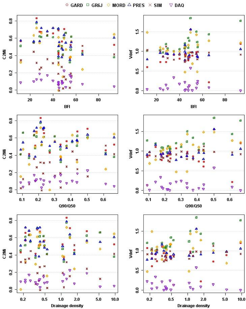
Figure 7: Relation between mean performance in simulation on the two validation periods in terms of C2Mi, (left) and Vdef (right), and catchment or streamflow characteristics (topleft: Base-Flow Index, centremiddle: Q_{90}/Q_{50} ratio; rightbottom: drainage density) for the 21 catchments and the models tested.
