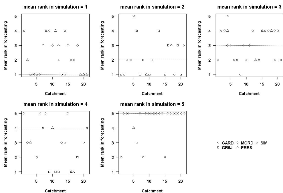
Figure 12: Mean model ranks for the 7-day in-forecasting at the 7-day lead-time for the 21 catchments for the models ranked 1 st , 2 nd , ..., 5 th in simulation.
