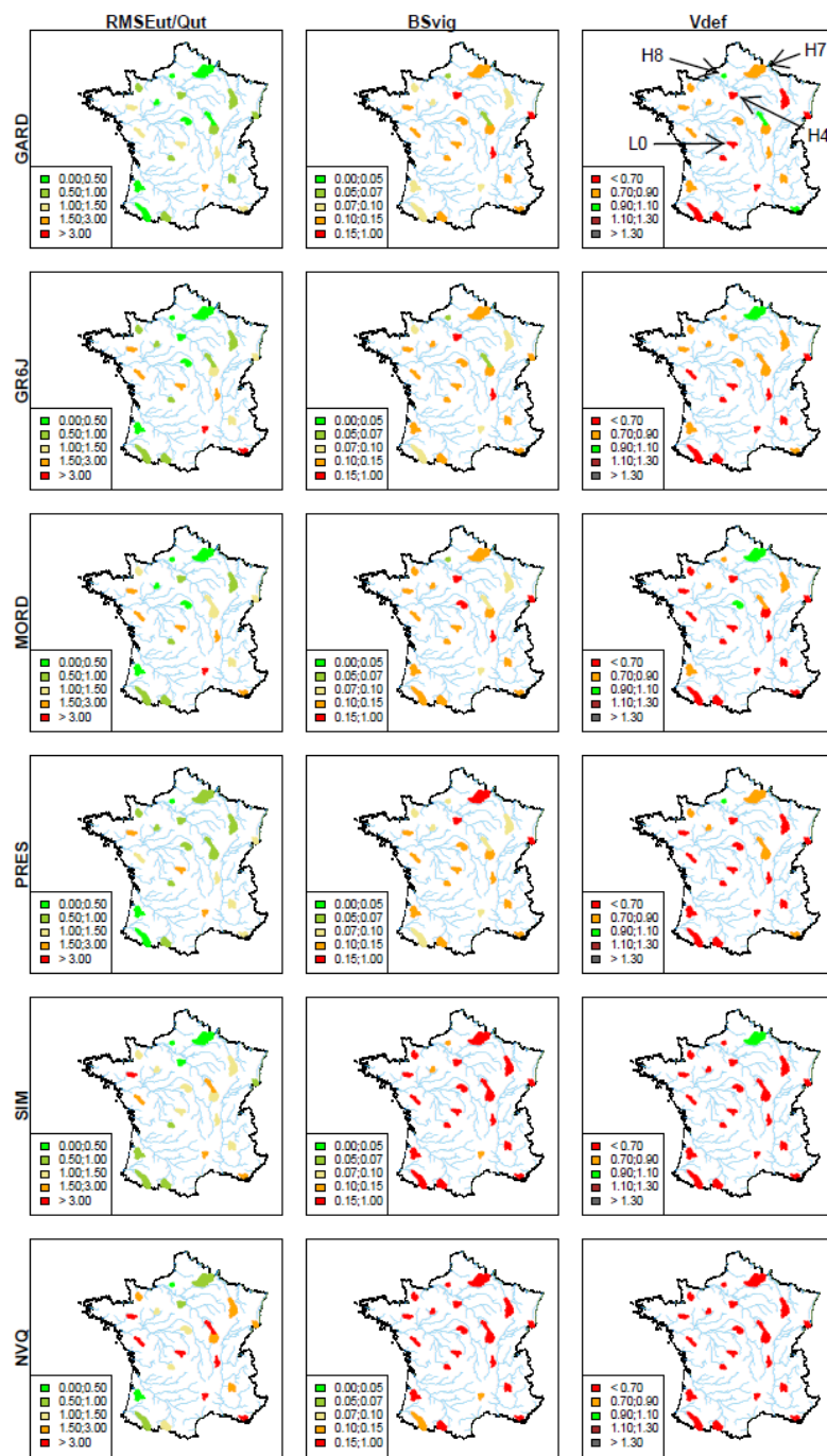
Figure 10: Model pPerformance in forecasting mode on validation period 2 for the RMSE ut/Out , BS vig and V def criteria for each model on the 21 catchments for a 7-day forecasting lead time. The letters on the top right map show the catchments (first two letters of the HYDRO code, see Table 1) whose results are commented in more details in the text (H4: Orge; H7: Oise; H8: Andelle; L4: Petite Creuse)
