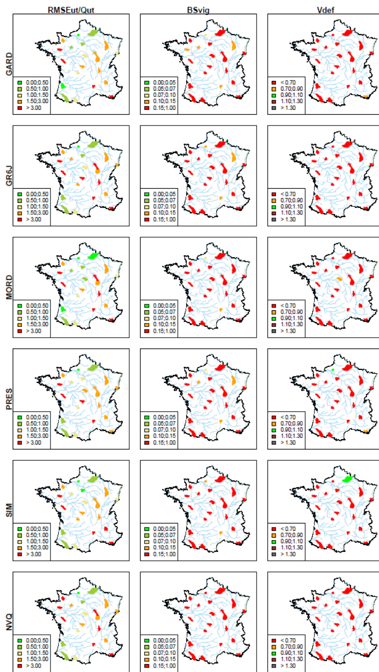
Figure 11: Model performance in forecasting mode on validation period 2 for the RMSE ut , BS vig and V def criteria for each model on the 21 catchments for a 30-day forecasting lead time
