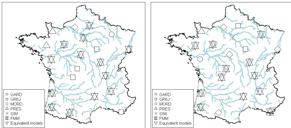
Figure 15: Maps of the model ranked best in simulation for the mean of all criteria and for validation periods 1 (left) and 2 (right), including the multi-model (fixed-weight average approach, FMM)
