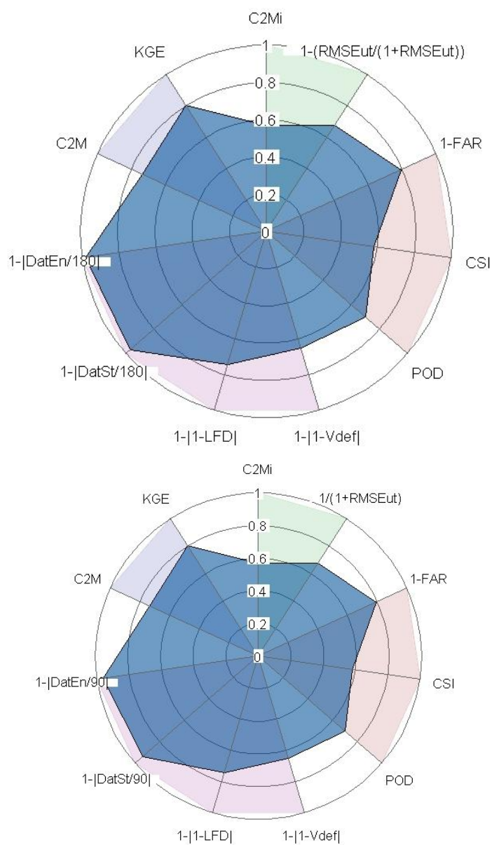
1190 Figure 3: Example of radial plot showing mean model results on the set of 21 catchments for the selected evaluation criteria. The larger the blue surface, the better the model. Background colours link criteria focusing on similar aspects
