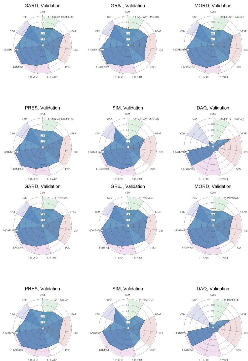
Figure 4: Radial plots showing the mean validation results obtained by the five tested models and the benchmark (DAQ) for the selected criteria in validation for over the 21 catchments and the two test periods, in simulation mode. Results of the five models tested and the benchmark (DAQ) are shown.
