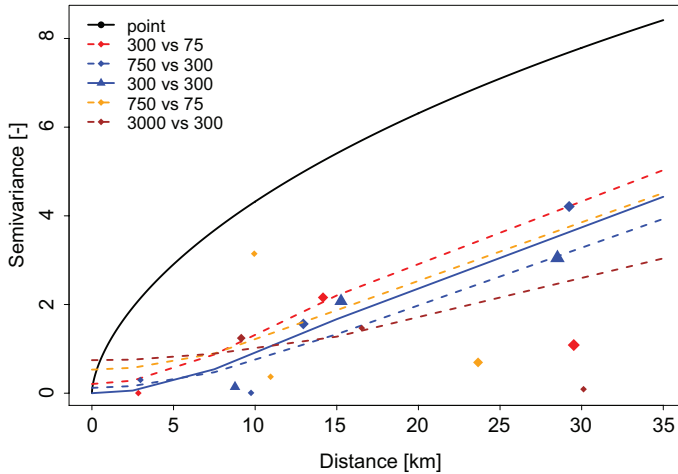
Fig. 4. Sample variogram (points) and regularized variograms as function of distance and area. The black solid line represents the fitted point variogram, the blue line represents regularized variogram of equally sized catchments ( \sim 300 \text{ km}^2 ), dotted lines show the effect of combinations of different catchments sizes in square kilometers (see also Fig. 4 in Skøien et al., 2014).
