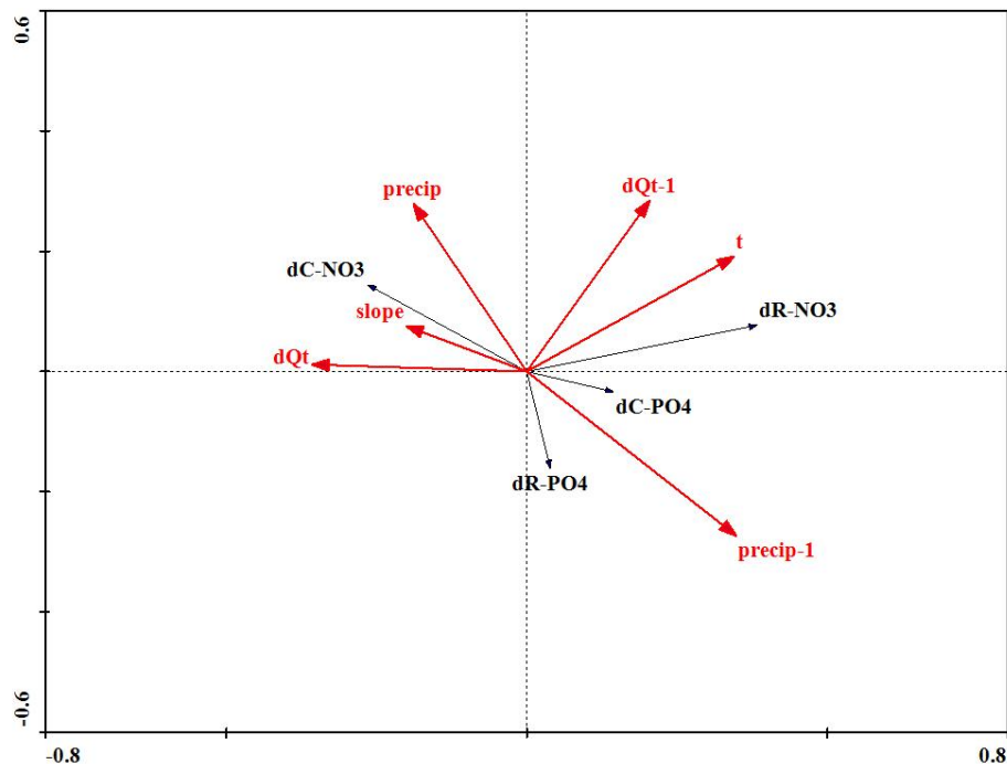
Fig. 10. RDA analysis ordination diagram – the impact of hydrological parameters on concentration values and formation of hysteresis loops by using the parameters STABLE and INF as covariates (used labels is same as in Fig. 9)
