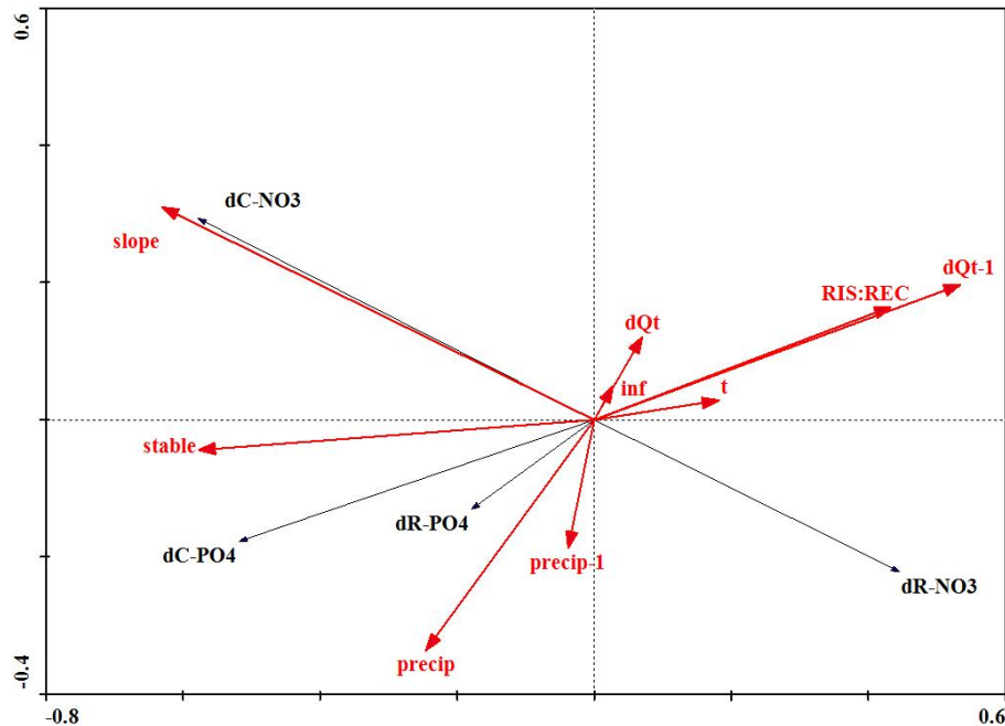
Fig. 11. RDA analysis ordination diagram – the impact of hydrological parameters on concentration values and formation of hysteresis loops during summer rainfall-runoff events (1 April–31 October) (used labels is same as in Fig. 9).
