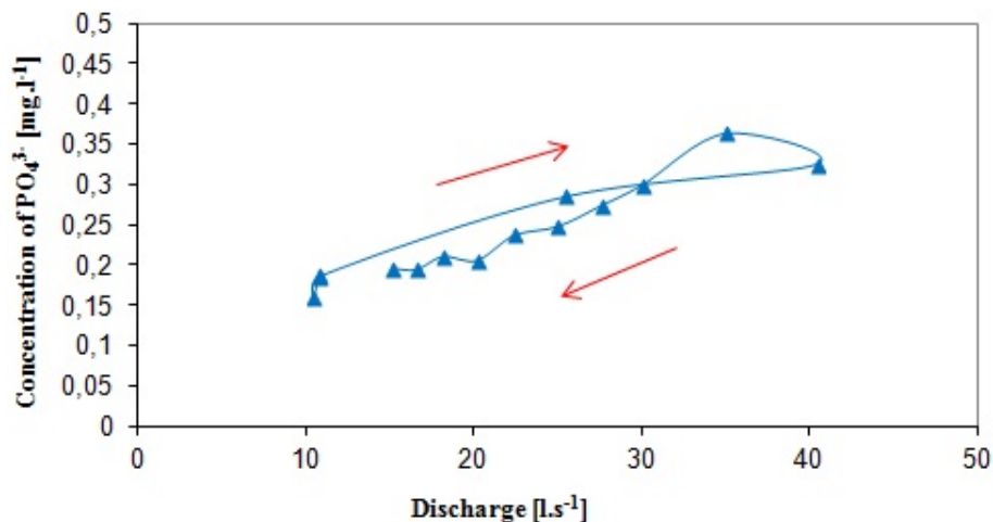
Fig. 7. Preview of hysteresis loop formation for phosphate anions PO_4^{3-} for rainfall-runoff event recorded on the 24–25 June 2009 in the subcatchment J2 in Jenínský stream catchment; arrows indicate the time course of the event.
