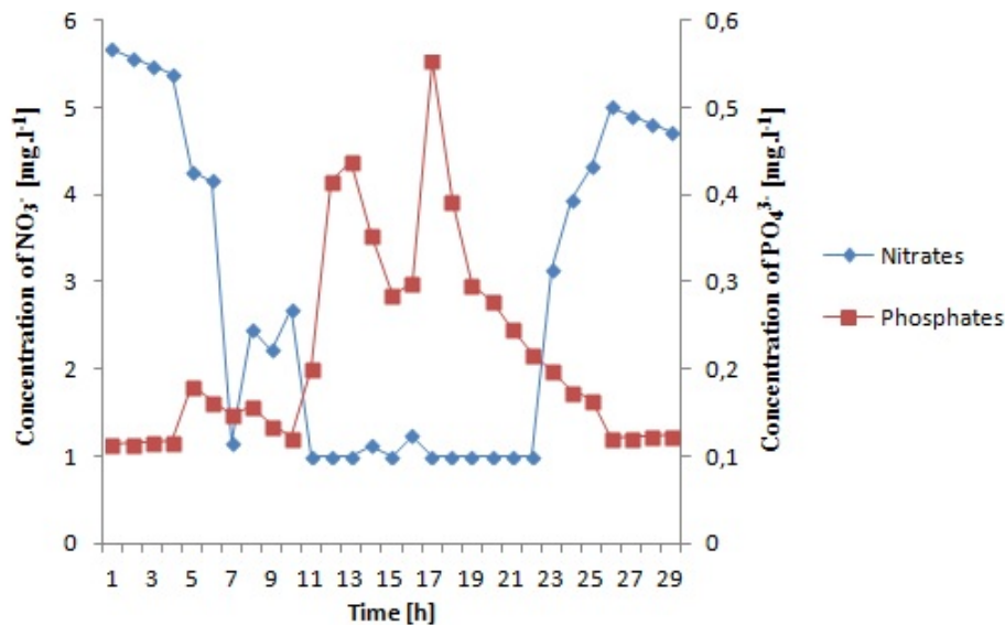
Fig. 8. Development of nitrate and phosphate anions concentration during rainfall-runoff events in the Jenínského stream catchment (J2) from 13–15 May 2010.
