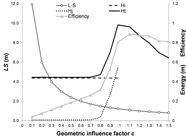
Fig. 7. Profiles of the main energetic parameters as a function of the geometric influence factor c for initial conditions ( q = 0.5 \text{ m}^2 \text{ s}^{-1} ; S = 5\% ; n = 0.04 ; z = 1.19 ). E_{fs} = efficiency in the reduction of friction slope; H_i = energy dissipated at the impact zone; H_j = energy dissipated at the hydraulic jump; H_t = total energy dissipated ( H_i + H_j ); LS = difference in total head between adjacent dams.
