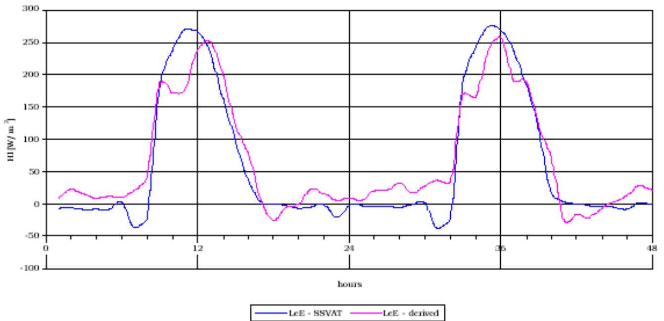
Fig. 9. Latent heat derived from turbulent measurements and simulated by the SSVAT model – period: 8-9 October 1999.
