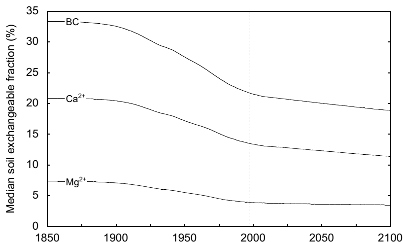
Fig. 8. Simulated median soil exchangeable fractions for calcium (Ca 2+ ), magnesium (Mg 2+ ) and base cations (BC) during the period 1850–2100. The broken line separates hindcast and forecast simulations.
