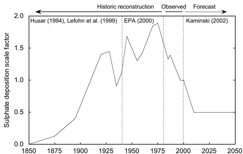
Fig. 2. Estimated historic and future sulphate deposition (scale factor; 1997 deposition (41 μmol c L -1 ) is equivalent to a factor of 1.0) for the period 1850–2050. The broken lines separate the different data sources used to construct the deposition sequence.
