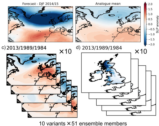
Figure 2. Schematic outlining the Historic Weather Analogues method for an example winter (2014/2015). Panel (a) shows GloSea forecast of standardised sea level pressure (SLP) anomalies over winter 2014/2015. Panel (b) shows the mean SLP anomalies across all 510 historical weather analogues ensemble members. Panel (c) shows the SLP anomalies of five example analogue variants where each variant is made up of three months from different historical years (i.e. December 2013/January 1989/February 1984). Panel (d) shows the average rainfall across the UK from the five example analogue variants. The analogue sampling contains ten analogue variants per ensemble member and is repeated for each of the 51 ensemble members of GloSea5 with a total of 510 analogue forecasts.
