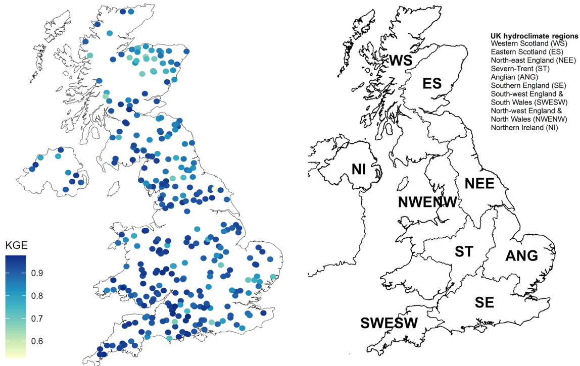
Figure 1. Model performance based on the modified Kling-Gupta efficiency (KGE) calculated from square root transformed simulated river flows (left) and the nine UK hydroclimate regions used to aggregate and summarise skill score results (right).
