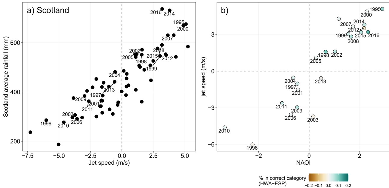
Figure 10. Linking winter river flow predictability to atmospheric circulation patterns. (a) Scotland average rainfall against mean winter North Atlantic jet speed ( \text{m s}^{-1} ) for 1956–2018, with the years in the hindcast period highlighted. Panel (b) shows jet speed ( \text{m s}^{-1} ) against the North Atlantic Oscillation (NAO) index, with the dots coloured by the percentage of HWA forecasts in the correct category as the retrospective simulation minus the percentage of ESP forecasts in the correct category as the retrospective simulation averaged across catchments in Scotland for all years in the hindcast period – positive values indicate a higher percentage of forecasts in the correct category in HWA compared to ESP.
