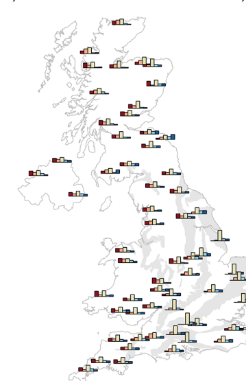
Figure 9. Case studies from the hindcast experiment for DJF 1994/1995 (top) and 2009/2010 (bottom). ESP hindcasts are shown in the left panels, with HWA hindcasts in the central panels, and the river flow category for retrospective simulated river flows flows in the rightmost panels. Note the visualisation style is the same as the operational UK Hydrological Outlook and in the interactive online portal. The colour scheme has been adopted after extensive stakeholder consultation.
