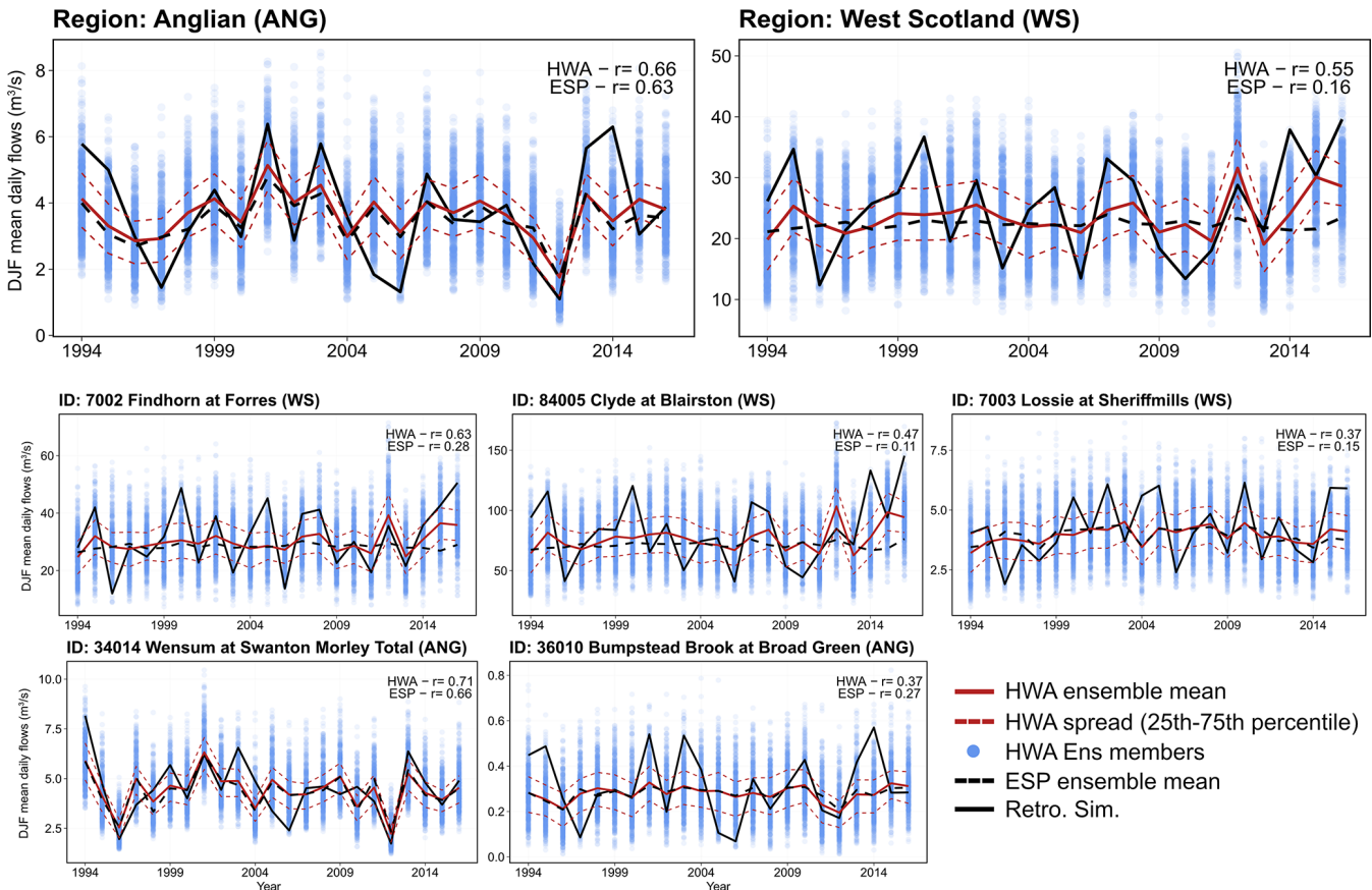
Figure 6. December–January–February (DJF) mean daily simulated flows ( \text{m}^3 \text{s}^{-1} ) averaged across catchments in two contrasting regions (West Scotland and Anglian) and for five individual example catchments with varying skill in each region. Blue dots show the individual ensemble members from the HWA method, the red solid line shows the HWA ensemble mean, the red dotted lines show the HWA spread (25th–75th percentile), the dotted black line shows the ensemble mean of the standard ESP method and the solid black line shows retrospective simulated river flows. The correlation coefficients between the retrospective simulated river flows and the ensemble mean HWA and ESP forecasts are shown on each plot.
