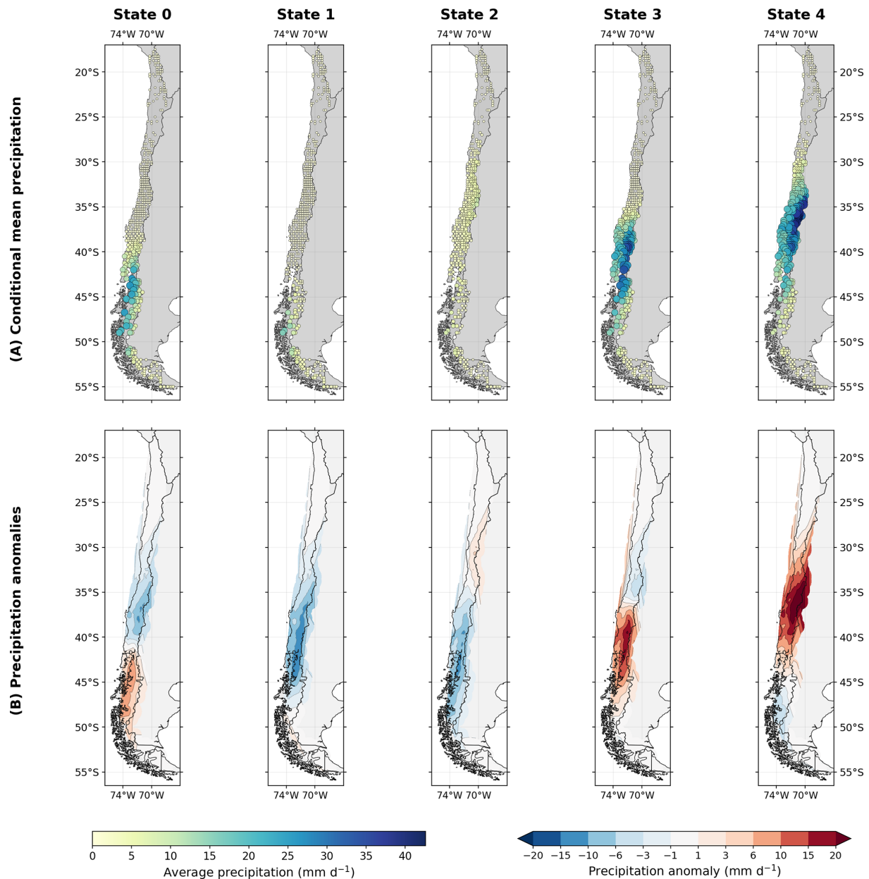
Figure 1. Mean precipitation and anomalies by nHMM state (MJJA, 1980–2021). (A) Conditional mean daily precipitation ( \text{mm d}^{-1} ) across the 462 locations for each of the five latent states; marker size and colour are proportional to the conditional mean. (B) Precipitation anomalies ( \text{mm d}^{-1} ) relative to the MJJA climatology, shown as full-size interpolated maps for readability. States “0”/“1”: dry regimes; “2”: transitional; “3”/“4”: wet regimes, strongest over \approx 35 – 45^\circ S.
