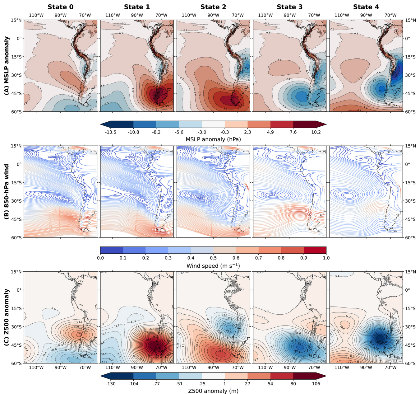
Figure 2. Circulation composites by nHMM state (MJJA, 1980–2021). (A) Mean sea-level pressure (MSLP) anomalies (hPa) relative to the MJJA climatology; (B) 850 hPa wind streamlines, coloured by normalized wind speed; (C) 500 hPa geopotential height (Z500) anomalies (m). Contour labels indicate anomaly magnitudes. Dry regimes (e.g., State 1): ridge–high couplet with weakened westerlies. Wet regimes (e.g., State 4): trough–low couplet with an intensified westerly jet impinging on central–southern Chile.
