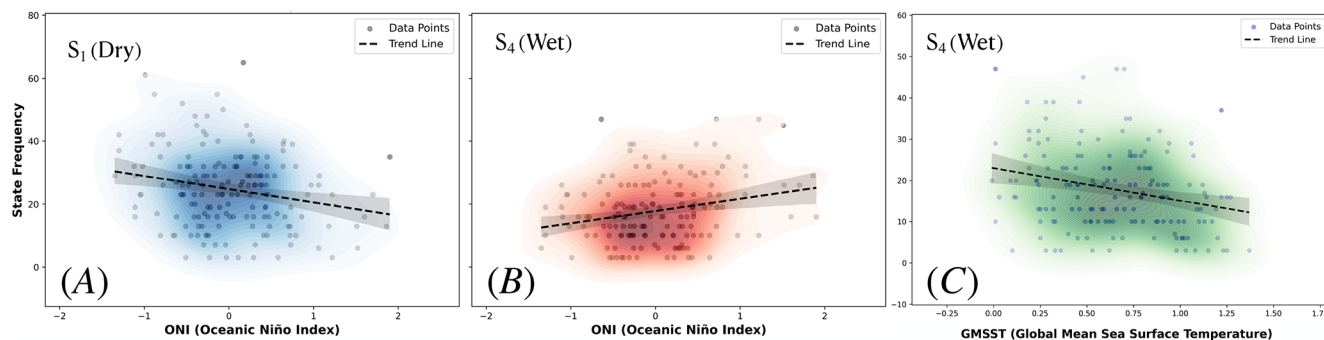
Figure 5. State-index relationships (MJJA, 1980–2022). (A) ONI vs monthly frequency of the dry state f_1 ; (B) ONI vs f_4 ; (C) GMSST vs f_4 . Kernel-density contours; dashed: OLS fits with 95 % bands (descriptive only). Tail-enhanced associations motivate copula-based nonlinear dependence modelling.
