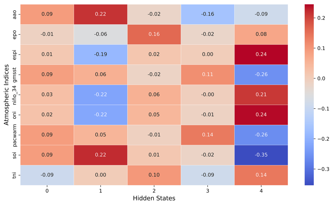
Figure 4. Pearson correlations between seasonal state frequencies and atmospheric indices (MJJA, 1980–2022). Asterisks: significant at the 5 % level after effective-sample-size correction (Pyper and Peterman, 1998). Signs agree with ENSO modulation; moderate magnitudes are consistent with teleconnections that modulate – not deterministically control – synoptic regimes.
