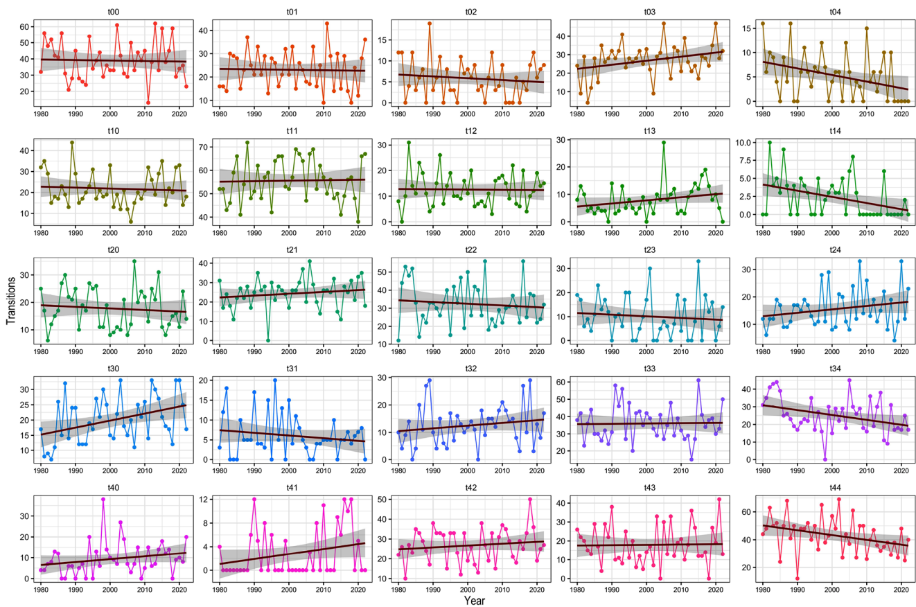
Figure 3. Annual transition proportions and Generalized Linear Mixed Model (GLMM) trends (MJJA, 1980–2022). Points: annual proportions p_{ij}^{(y)} . Solid lines: logit-linear GLMM trends (minimum 25 nonzero years, \sum_y C_{ij}^{(y)} \geq 100 ). Shaded bands: 95 % CIs. Red dashed: significant trend after BH-FDR correction ( p < 0.05 ).
