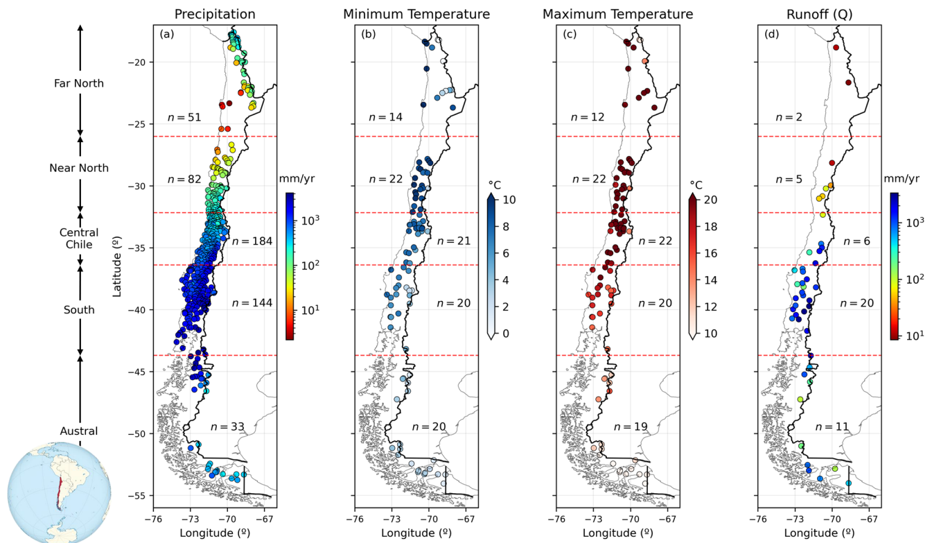
Figure 1. Temporal averages of (a) annual precipitation, (b) minimum daily temperature, (c) maximum daily temperature, and (d) annual runoff measured at stations over the period April/2001–March/2018. Annual means were computed considering only water years with at least 80 % data availability. Red dashed lines indicate the boundaries of the study macrozones.
