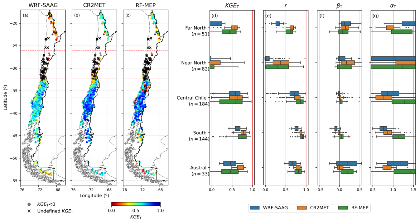
Figure 5. (a–c) Spatial distribution of Tang’s Kling–Gupta Efficiencies ( KGE_T ) for summer (DJF) daily precipitation retrieved from WRF-SAAG, CR2MET, and RF-MEP (period April/2001–March/2018) across continental Chile, using ground-based observations as the reference. Red dashed lines indicate the limits of the macrozones analyzed. (d–g) Boxplots with KGE_T , the Pearson correlation coefficients ( r ), bias term ( \beta_T ), and variability ratios of Tang’s Kling–Gupta Efficiency ( \alpha_T ) obtained with the products examined for each macrozone, with the red line indicating the optimal value. Each boxplot comprises results for all the stations within a specific macrozone. The boxes correspond to the interquartile range (IQR, i.e., 25th and 75th percentiles); the vertical line in each box is the median, and the whiskers extend to the \pm 1.5 \cdot \text{IQR} of the ensemble of stations.
