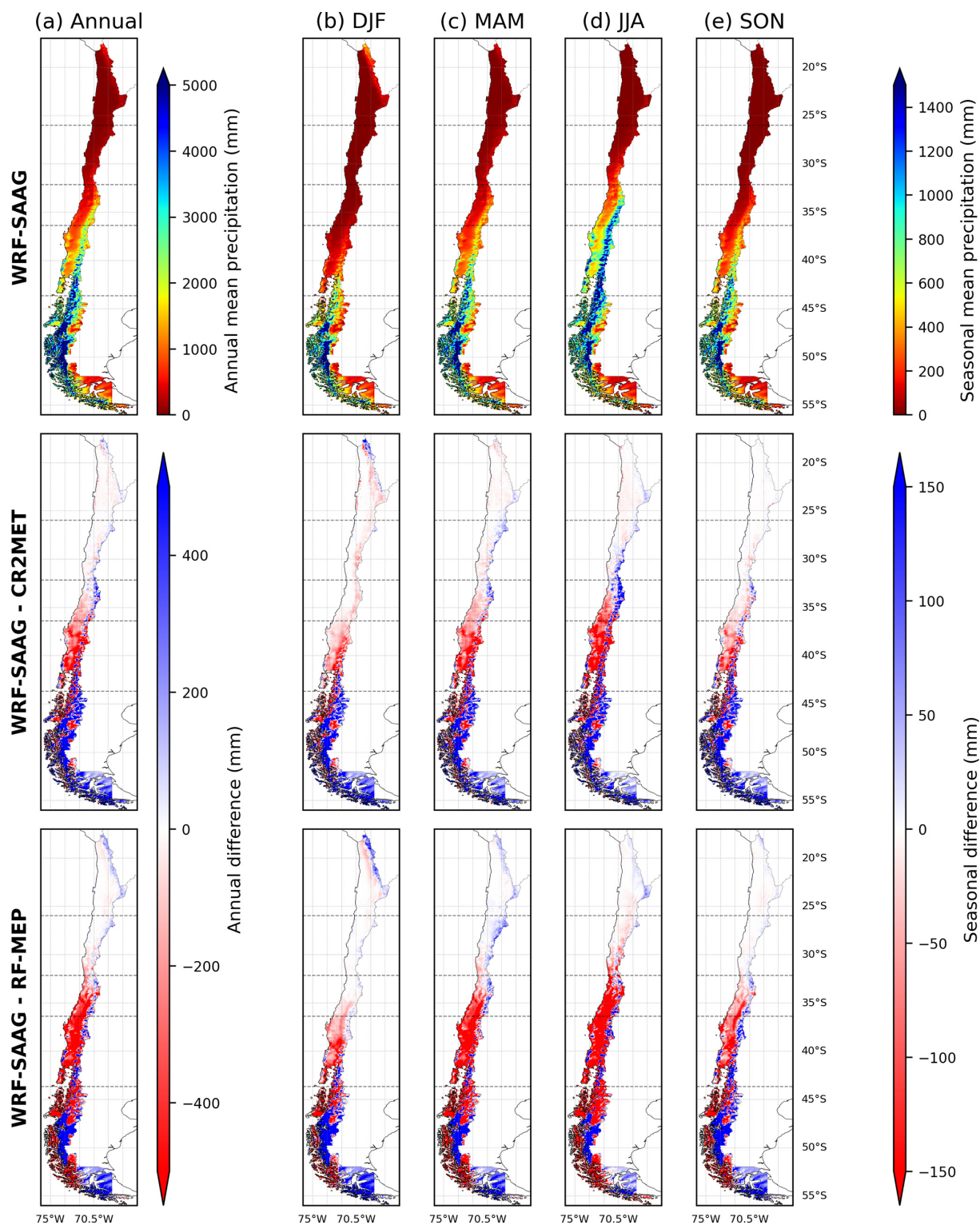
Figure 2. Spatial distribution of mean precipitation simulated by WRF-SAAG and precipitation differences relative to CR2MET and RF-MEP over Chile (April/2001–March/2018). Columns show (a) annual means and seasonal means for (b) summer, (c) autumn, (d) winter, and (e) spring. The top row displays mean precipitation from WRF-SAAG, while the middle and bottom rows show precipitation differences between CR2MET and WRF-SAAG, and between RF-MEP and WRF-SAAG, respectively. Horizontal dashed lines indicate the boundaries of the five latitudinal macrozones: Far North, Near North, Central Chile, Southern, and Austral.
