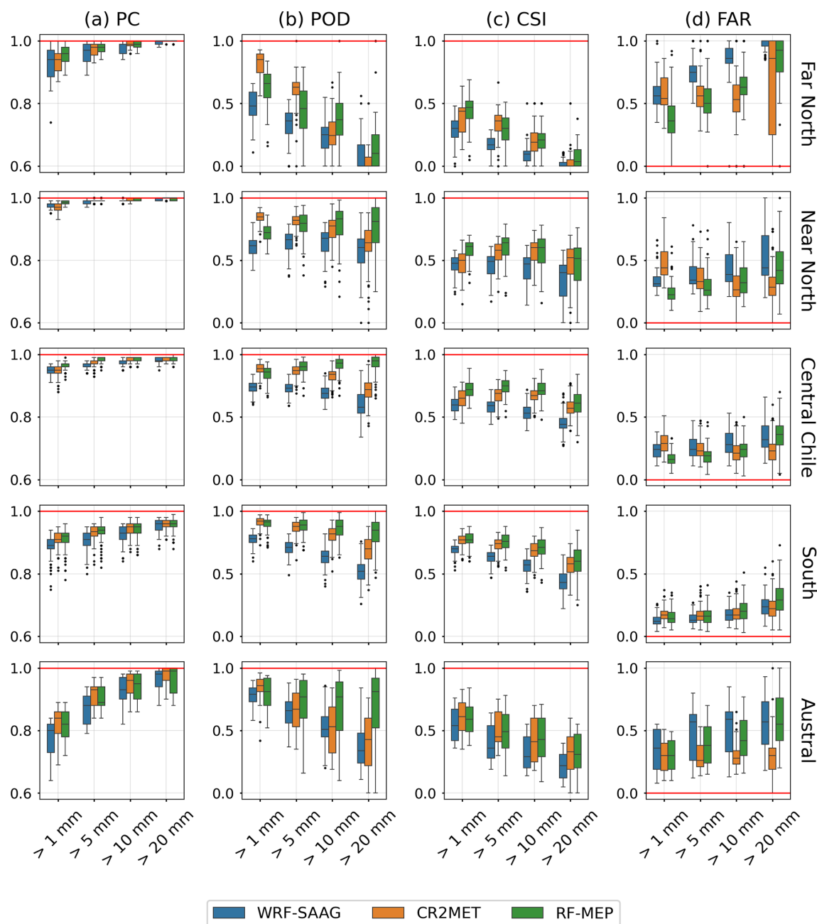
Figure 4. Ability of WRF-SAAG, CR2MET, and RF-MEP to replicate historically observed daily precipitation events with amounts larger or equal than 1, 5, 10, and 20 mm d -1 in the study macrozones (rows). The metrics displayed in each column are: (a) Percentage Correct (PC), (b) Probability of detection (POD), (c) Critical Success Index (CSI), and (d) False Alarm Ratio (FAR). Each boxplot comprises results from all the stations within each macrozone. The boxes correspond to the interquartile range (IQR, i.e., 25th and 75th percentiles), the horizontal line in each box is the median, and whiskers extend to the \pm 1.5 \cdot \text{IQR} of the ensemble. The red line represents the optimal values.
