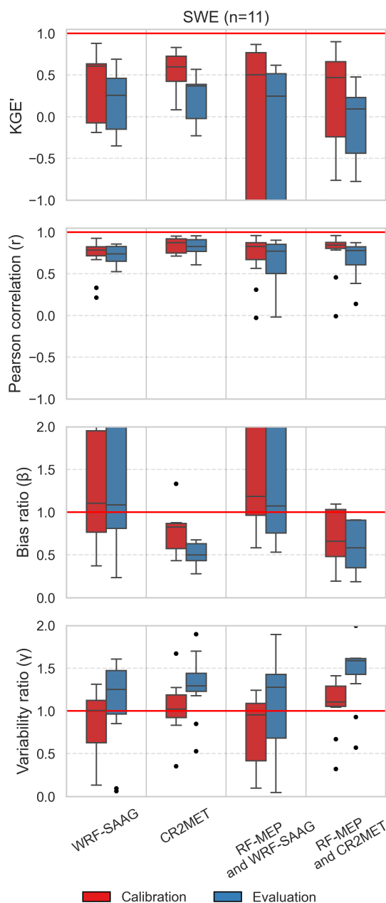
Figure 13. Evaluation of snow water equivalent (SWE) simulated with the TUW model during the calibration (April/2005–March/2011) and the first four years of the evaluation period (April/2011–March/2015) for 11 case-study basins, using different input forcing combinations: WRF-SAAG (precipitation and temperature); CR2MET (precipitation and temperature); RF-MEP (precipitation) with WRF-SAAG (temperature); and RF-MEP (precipitation) with CR2MET (temperature). Each boxplot includes five basins located in the Near North macrozone, five basins in Central Chile, and one basin in the Southern macrozone. The boxes represent the interquartile range (IQR; i.e., the 25th and 75th percentiles), the horizontal line within each box indicates the median, and the whiskers extend to \pm 1.5 \cdot \text{IQR} across the ensemble of stations. Please note that the evaluation period is shorter than the one used for ET and soil moisture since the reference SWE data set covers until March/2015.
