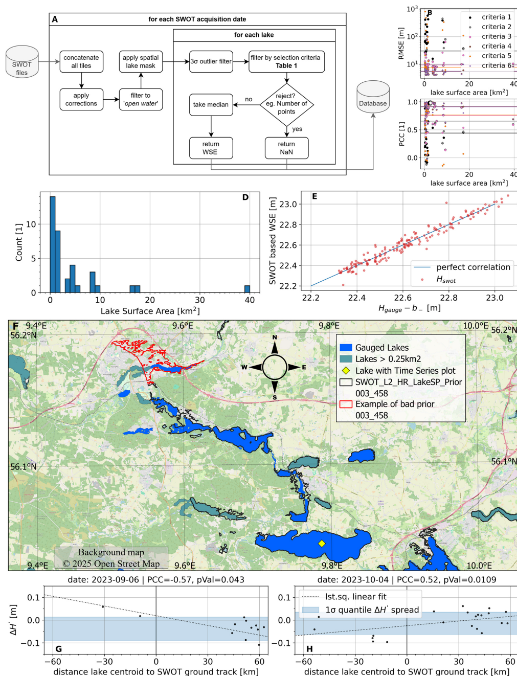
Figure A1. (A): flowchart of method pipeline. (B) and (C): RMSE and PCC for all lakes and all selection criteria over lake surface area. (D): distribution of lake surface area of all 37 lakes in this study. (E): correlation scatter plot for Mossø, shown in Fig. 3C. (F): Example of prior problem in LakeSP for Danish lakes around Viborg. (G) and (H): Example of two acquisition without significant residual roll error: error over distance to SWOT ground track.
