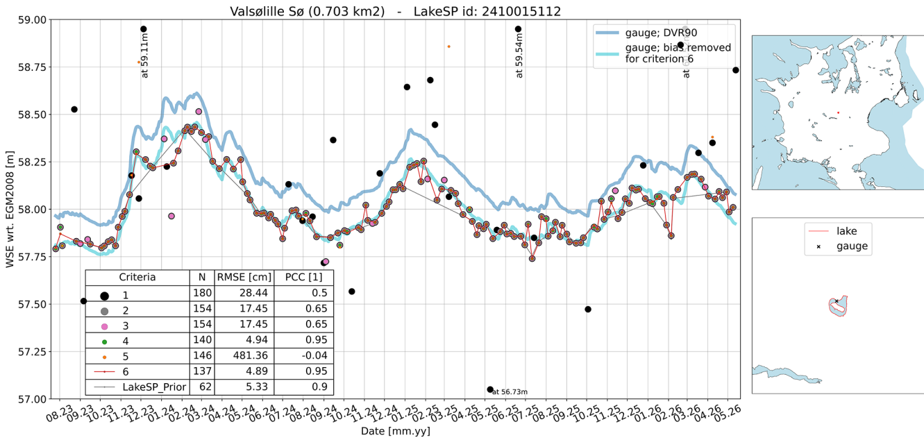
Figure 2. SWOT WSE time series for all 6 defined data selection criteria, exemplary for Valsølle Sø, with RMSE and Pearson Correlation Coefficient vs. gauge data and the number of timestamps in the respective time series ( N ). Filtered LakeSP prior data is shown for reference.
