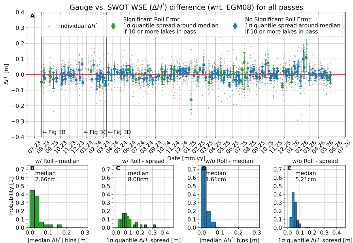
Figure 6. (A): \Delta H' (SWOT vs. gauges) over time for all passes and all lakes in Denmark. For timestamps with \geq 10 observed lakes, the median and 1\sigma quantile spread (0.1585 to 0.8415) are shown. If \Delta H' significantly correlates with distance to SWOT's ground track ( d ), it is shown in green, otherwise in blue. The three vertical lines indicate the timestamps with detailed correlation plots in Fig. 5B–D. (B): distribution of the absolute median \Delta H' for timestamps with significant roll error. (C): distribution of the 1\sigma quantile spread for timestamps with significant roll error. (D): distribution of the absolute median \Delta H' for timestamps without significant roll error. (E): distribution of the 1\sigma quantile spread for timestamps without significant roll error.
