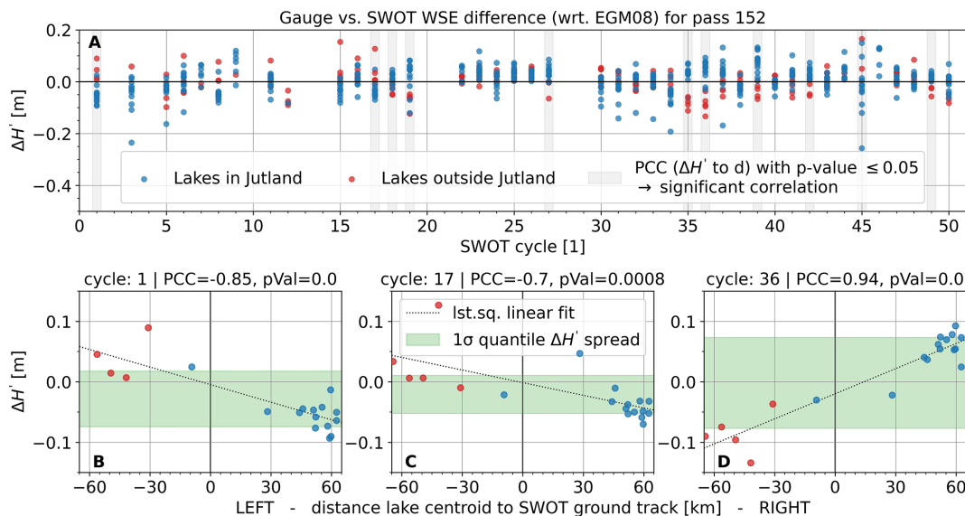
Figure 5. (A): \Delta H' (SWOT vs. gauges) over time for all lakes in pass 152. (B)–(D): expanded plot of SWOT's error per lake over lake's centroid distance to SWOT's ground track. Negative distances are left and positive to the right of SWOT. Exemplary for the cycles 1, 17, and 36.
