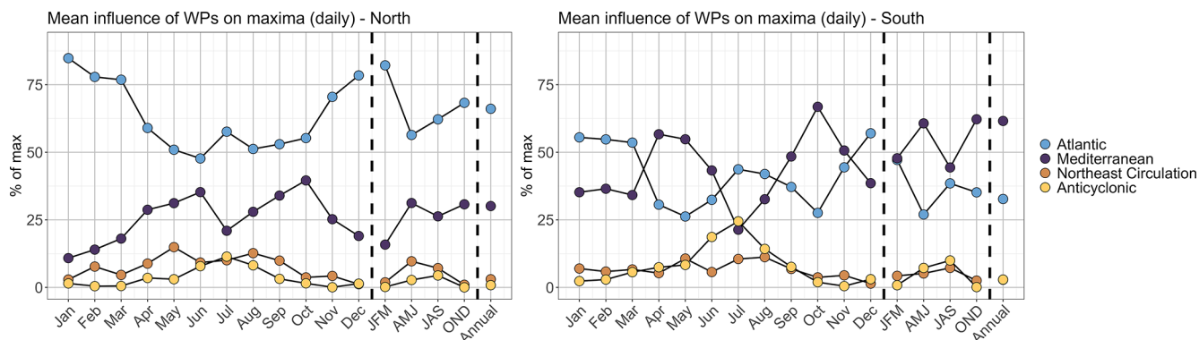
Figure 6. Relative influence of the four weather patterns on monthly/seasonal/annual maxima of daily precipitation intensity in the study region, for the period 1980–2023 grouped by stations north (left) and south (right) of the climatological divide.
