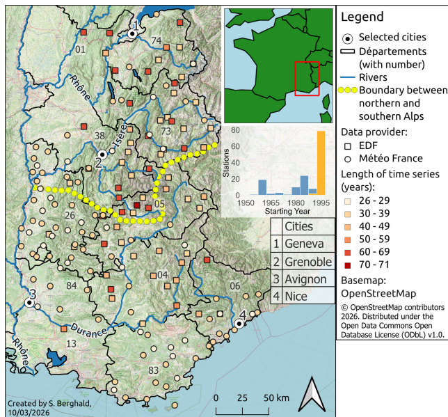
Figure 1. Study area and locations of precipitation observations used in this study. Stations maintained by Météo-France are shown as circles, and are used for stationary analysis only due to the comparatively short period they have been operating for. Stations maintained by EDF are shown as squares, and are used for both the stationary and the trend analysis (see Sect. 2.2.4). The colour of a point indicates the length of the hourly time series in years (including data from the “old” dataset where available). The length of daily time series is not shown, but frequently exceeds the length of hourly data. The boundaries of the administrative regions ( départements ) are shown in black with their respective codes (see text). Important rivers are indicated in blue, and selected cities as black dots. The yellow line shows the climatological boundary between northern and southern Alps (Blanchard, 1921; Auer et al., 2007). First inlet: Position of the study area within France. Second inlet: Distribution of starting years for all stations (blue: EDF, yellow: Météo-France). Basemap: © OpenStreetMap contributors, (2025), OpenStreetMap, hillshade: Esri (2025).
