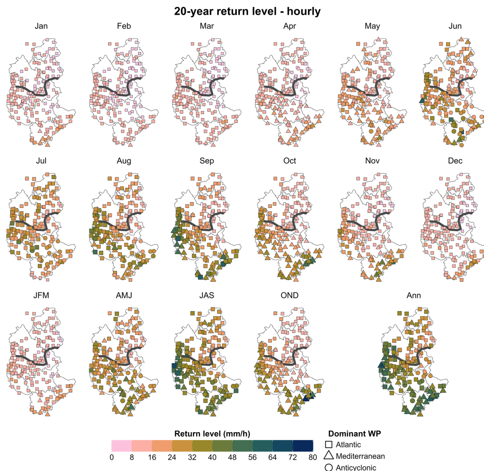
Figure 7. 20-year return levels of hourly precipitation extremes for EDF and Météo-France stations for the “recent” period (1980–2023). The colourscale and the size of the dots correspond to the amplitude of the 20-year return levels, the symbols to the dominant weather pattern. First and second row: monthly; third row: seasonal and annual.
