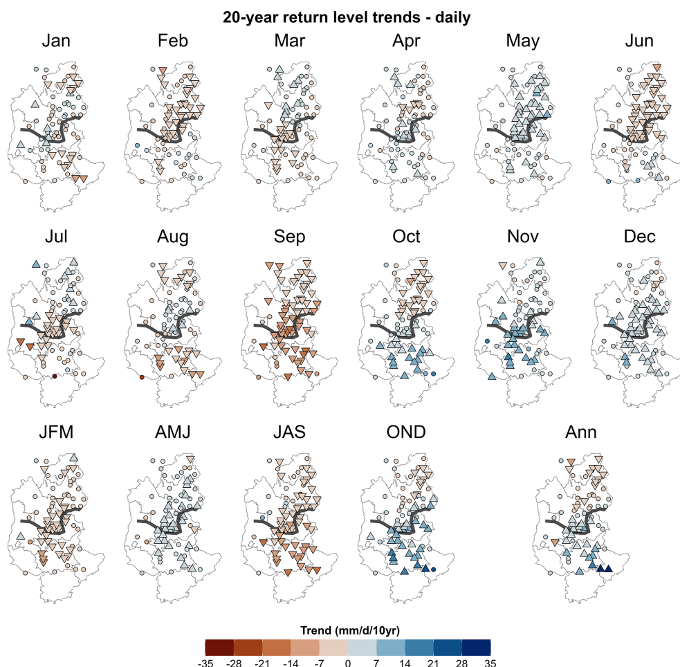
Figure 8. Trends of 20-year return levels of daily precipitation intensity between 1985 and 2022 using the nonstationary framework with a neighbourhood approach. Upward triangles indicate significant positive, downward triangles significant negative trends, and round points non-significant trends (positive and negative). First and second row: monthly; third row: seasonal and annual.
