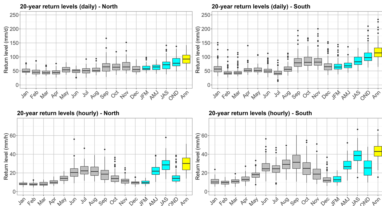
Figure 5. 20-year return levels of daily (first row) and hourly (second row) precipitation extremes for EDF and Météo-France stations for the 'recent' period (1980–2023), grouped into stations north (left column) and south (right column) of the climatological divide.
