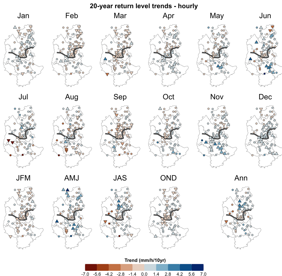
Figure 10. Trends of 20-year return levels of hourly precipitation intensity between 1985 and 2022 using the nonstationary framework with a neighbourhood approach. Upward triangles indicate significant positive, downward triangles significant negative trends, and round points non-significant trends (positive and negative). First and second row: monthly; third row: seasonal and annual.
