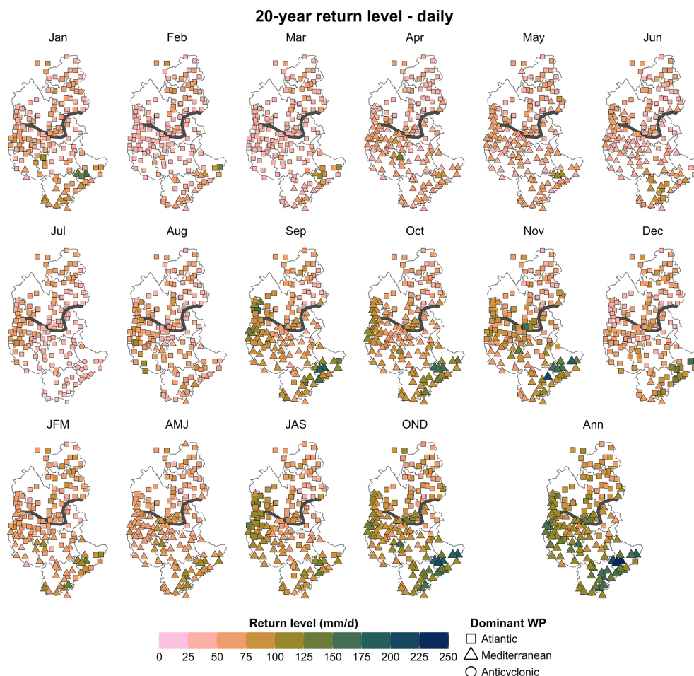
Figure 4. 20-year return levels of daily precipitation extremes for EDF and Météo-France stations for the “recent” period (1980–2023). The colourscale and the size of the dots correspond to the amplitude of the 20-year return levels, the symbols to the dominant weather pattern. First and second row: monthly; third row: seasonal and annual.
