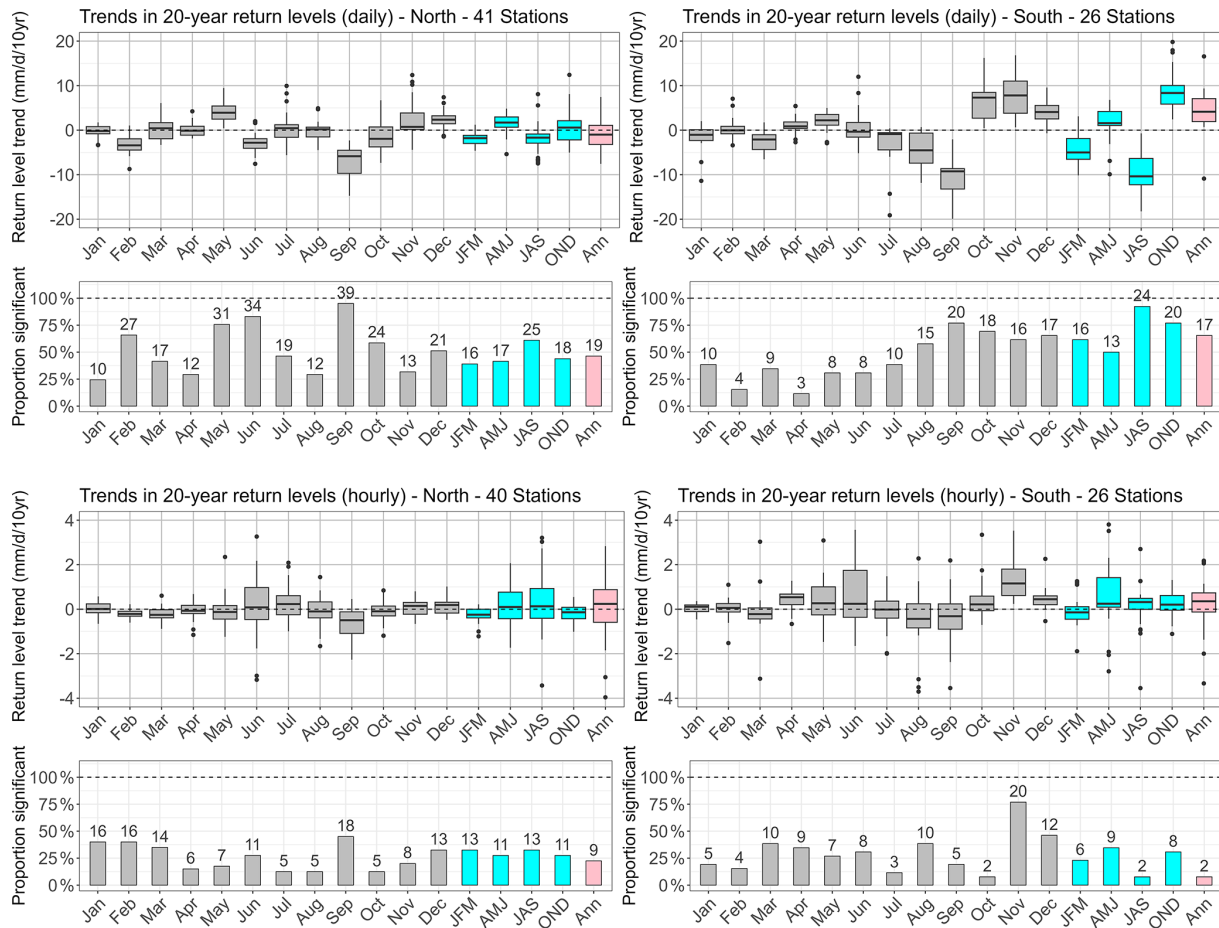
Figure 9. Trends of 20-year return levels of daily precipitation intensity between 1985 and 2022 using the nonstationary framework with a neighbourhood approach for daily (first row) and hourly (third row) precipitation extremes using all available time series of EDF stations (including “old” data) covering at least 34 years between 1952 and 2022 (66 of both hourly and daily data, 1 of daily data only). Both statistically significant and non-significant trends are included. The relative share and absolute number of stations with significant trends are shown in the second (daily) and fourth (hourly) row. The results are grouped into stations north (left column) and south (right column) of the climatological divide. For visualisation purposes the y-axis has been limited at \pm 20 \text{ mm d}^{-1}/10 \text{ years} for daily and at \pm 4 \text{ mm h}^{-1}/10 \text{ years} for hourly data, removing in total four daily and 16 hourly data points.
