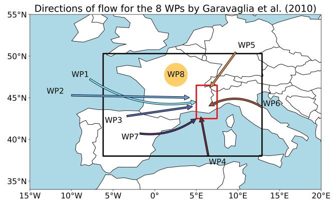
Figure 2. Direction of the large-scale flow directed to the study region for the eight weather patterns by Garavaglia et al. (2010) (WP8 groups anticyclonic conditions). The black box shows the area of interest for which the classification was done, and the red box shows the French Alps, the area of interest of this study. Figure adapted from Garavaglia et al. (2010, Fig. 3 therein).
