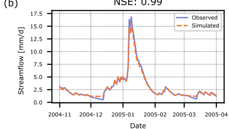
Model 5: Underparametrized model
