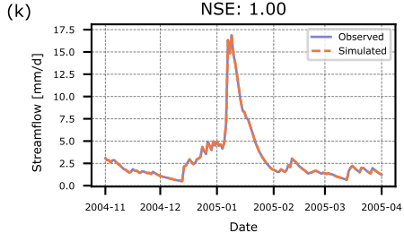
Model 8: Overparametrized Model
