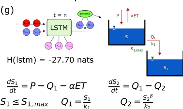
Model 7: Overparametrized model
