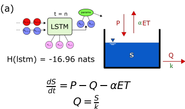
Model 5: Underparametrized model
