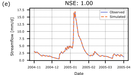
Model 6: Overparametrized model
