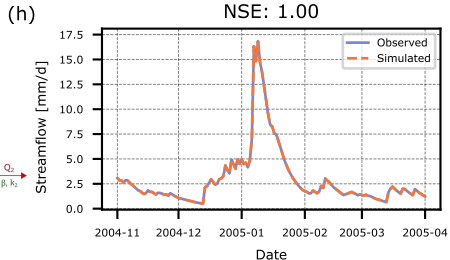
Model 7: Overparametrized model
