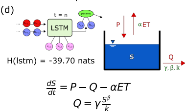
Model 6: Overparametrized model
