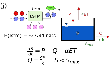
Model 8: Overparametrized Model
