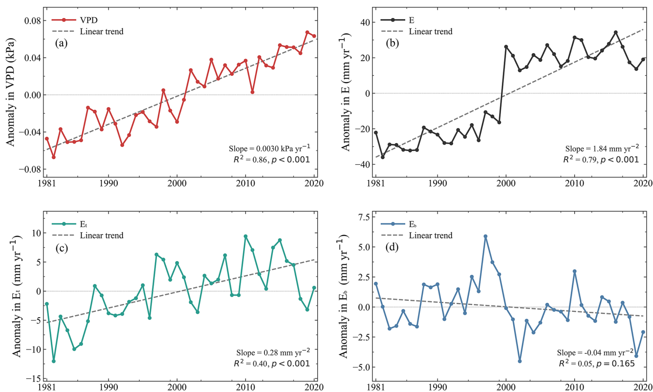
Figure 4. Interannual variability of global mean annual anomalies of VPD and evapotranspiration components during 1981–2020. (a) Global mean annual anomaly of vapor pressure deficit (VPD). The dashed line indicates the linear trend. (b) Global mean annual anomaly of total evapotranspiration ( E ). The dashed line indicates the linear trend. (c) Global mean annual anomaly of transpiration ( E_t ) over valid land pixels. The dashed line indicates the linear trend. (d) Global mean annual anomaly of bare-soil evaporation ( E_b ) over valid land pixels. The dashed line indicates the linear trend.
