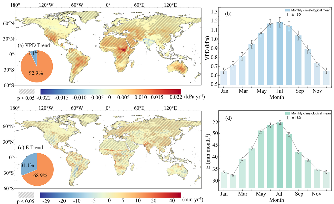
Figure 1. Spatial trends and seasonal cycles of terrestrial VPD and E during 1981–2020. (a) Sen's slope of VPD. Red colors indicate increasing trends, and blue colors indicate decreasing trends. Hatched areas indicate trends significant at p < 0.05 . The inset shows the percentages of valid land pixels with positive and negative VPD trends. (b) Global land monthly climatology of VPD during 1981–2020. Bars represent the climatological monthly means, circles indicate the corresponding mean values, and error bars represent \pm 1 standard deviation (SD) across years. (c) Sen's slope of terrestrial E . Red colors indicate increasing trends, and blue colors indicate decreasing trends. Hatched areas indicate trends significant at p < 0.05 . The inset shows the percentages of valid land pixels with positive and negative E trends. (d) Global land monthly climatology of E during 1981–2020. Bars, circles, and error bars are defined as in (b) . In the insets, orange indicates positive trends and blue indicates negative trends.
