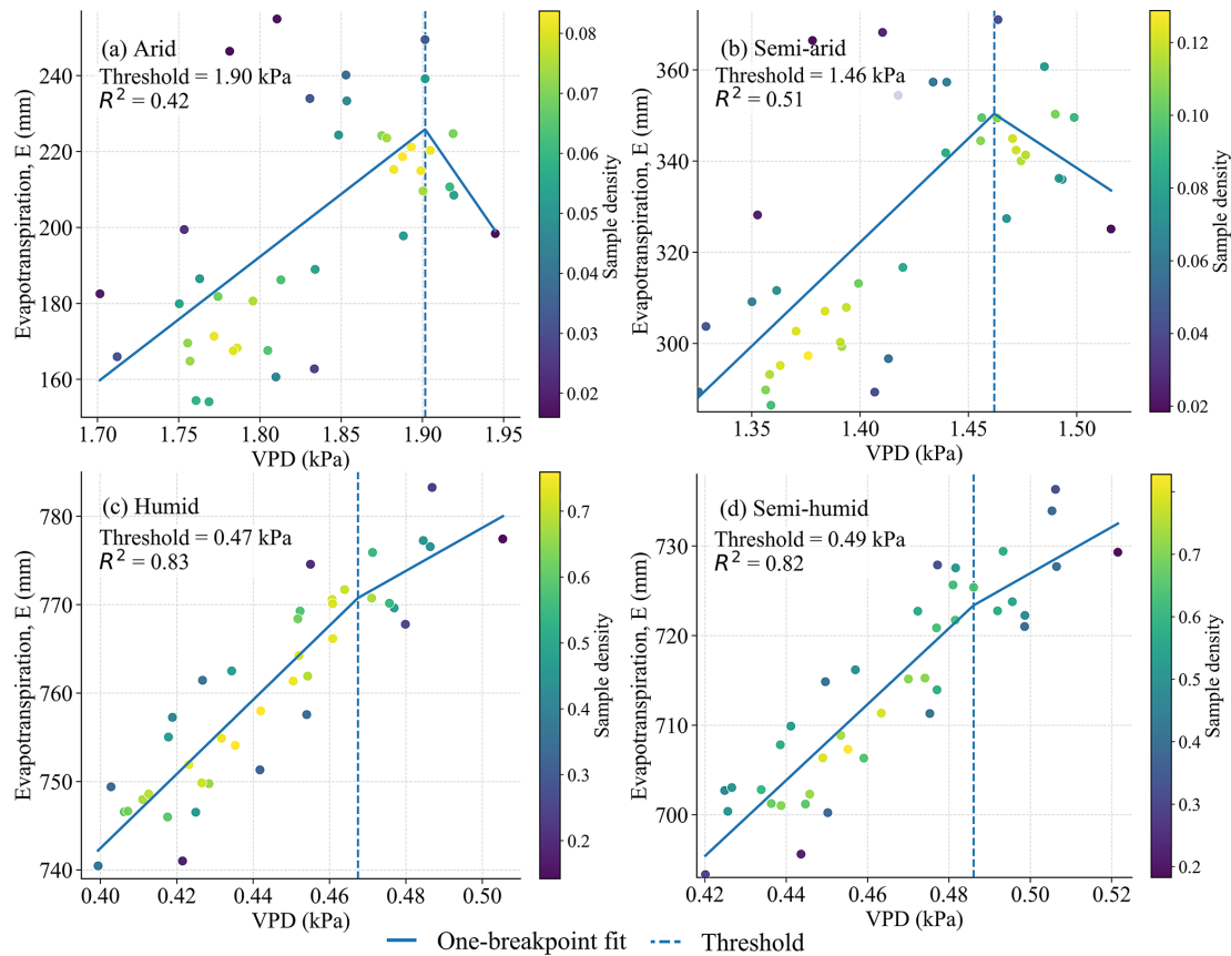
Figure 6. Aridity-dependent thresholds in the nonlinear response of terrestrial evapotranspiration to vapor pressure deficit. (a–d) One-breakpoint piecewise fits between VPD and E for the arid, semi-arid, humid, and semi-humid aridity zones, respectively. Points show annual area-weighted means, coloured by sample density. Solid lines indicate fitted relationships, and dashed vertical lines indicate the estimated VPD transition points. The AI-based aridity zones are shown in Fig. S5.
