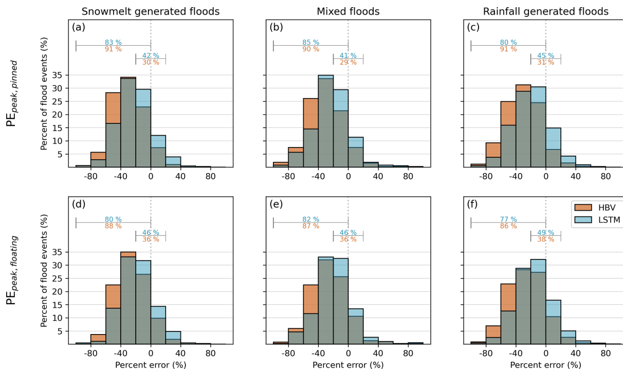
Figure 6. Percent error (PE) of flood peak magnitudes simulated by HBV (orange) and LSTM (blue) for the three different types of flood events: snowmelt generated floods (a, d), mixed floods (b, e) and rainfall generated floods (c, f). Upper panel (a–c) shows the pinned simulations ( PE_{peak,pinned} comparing discharge magnitudes at the day of observed peak), whereas lower panel (d–f) shows the floating simulations ( PE_{peak,floating} comparing observed peak discharge with maximum simulated discharge within 2 d of observed peak). In each subplot, the percentage of events that were underestimated (numbers at horizontal line extending -100\% to 0\% ), and the percentage of events with a relative error within \pm 20\% (numbers at horizontal line extending -20\% to 20\% ) are shown for LSTM (blue) and HBV (orange).
