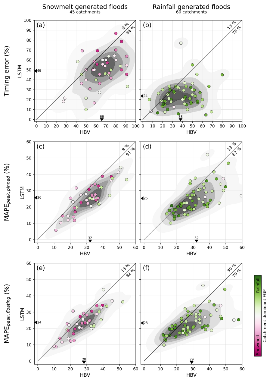
Figure 8. Flood peak performance scores per catchment for HBV ( x -axis) versus LSTM ( y -axis), for snowmelt generated floods (left) and rainfall generated floods (right). Upper panel (a–b) shows the peak timing error (percentages of incorrectly simulated days of peak discharges). Middle panel (c–d) and lower panel (e–f) show the mean absolute percentage error for pinned simulations ( \text{MAPE}_{\text{peak,pinned}} comparing discharge magnitudes at the day of observed peak), and for floating simulations ( \text{MAPE}_{\text{peak,floating}} comparing observed peak discharge with maximum simulated discharge within two days of observed peak), respectively. Background is shaded by the corresponding 2D empirical density function. Triangles with adjacent numbers represent catchment average score for each model. Dots below the diagonal line represent catchments with better (i.e. smaller error) metric values for LSTM as compared to HBV. The percentages of catchments above and below the diagonal lines are provided in the upper right corner of each scatterplot. Each catchment is coloured by the corresponding catchment’s dominant flood generating process (FGP, ref. Fig. 2).
