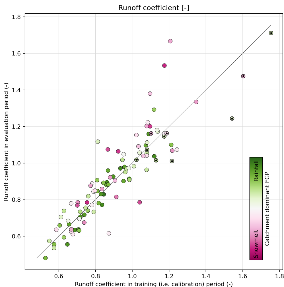
Figure C1. Runoff coefficient (i.e. ratio of streamflow ( \text{mm d}^{-1} ) to precipitation ( \text{mm d}^{-1} )) of each catchment in the training period (i.e. calibration period; x -axis) versus the evaluation period ( y -axis). A dot close to the diagonal line implies consistent runoff coefficients for the two periods. Catchments with glaciers covering more than 3 % of their area are marked with stars. We note that values exceeding 1 (i.e. streamflow larger than precipitation) are mainly due to underestimation of precipitation, although glacier melt can explain part of the difference in catchments with glaciers. Each catchment is coloured by the corresponding catchment's dominant flood generating process (FGP, ref. Fig. 2).
