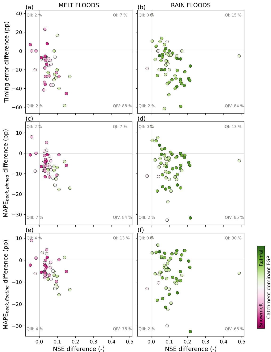
Figure C8. Model difference (i.e. LSTM minus HBV) in the overall performance metric NSE (x-axis) versus the flood peak metrics: (a–b) timing error, (c–d) \text{MAPE}_{\text{peak,pinned}} and (e–f) \text{MAPE}_{\text{peak,floating}} , separately for snowmelt generated floods (left) and rainfall generated floods (right). Each dot represents a catchment and is coloured by the catchment’s dominant flood generating process (FGP; ref. Fig. 2). Catchments within quadrant IV (QIV; lower right square) have a better score for LSTM as compared to HBV both in terms of overall performance score (NSE) and flood peak performance score. Percentages of catchments within each quadrant are given in the corners of the plots.
