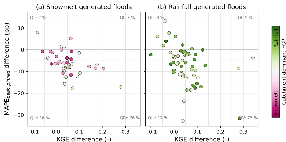
Figure 10. Model difference (i.e. LSTM minus HBV) in the overall performance metric KGE ( x -axis) versus the peak metric \text{MAPE}_{\text{peak,pinned}} ( y -axis) for (a) snowmelt generated floods and (b) rainfall generated floods. Each dot represents a catchment and is coloured by the catchment dominant flood generating process (FGP; ref. Fig. 2). Catchments within quadrant IV (QIV; lower right square) have a better score for LSTM as compared to HBV both in terms of overall performance score and flood peak performance score. Percentages of catchments within each quadrant are given in the corners of the plots.
