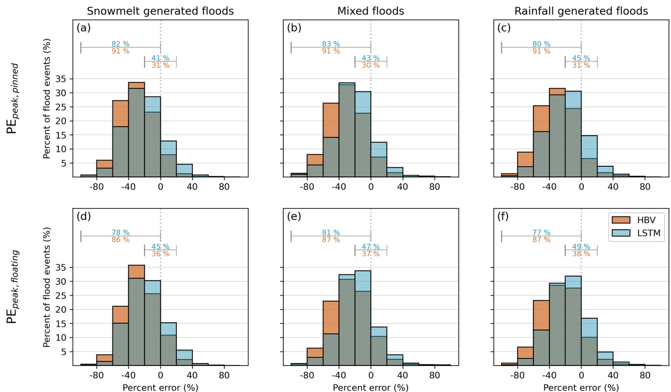
Figure C6. As Fig. 6, but using the alternative symmetric thresholds 0.2 and 0.8 for flood type classification (see Fig. C3).
