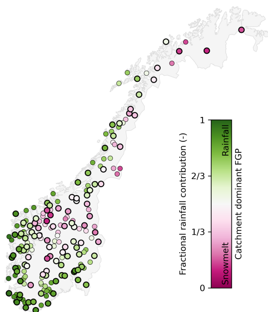
Figure 2. Average fractional rainfall (i.e. proportion of total) contribution to all observed flood events in the period 1 September 1994–31 August 2024, and its relation to the catchment dominant flood generating process (FGP). Dark pink (green) dots represent catchments with snowmelt (rainfall) as their dominant FGP, whereas near-white dots represent catchments with similar average contributions from rainfall and snowmelt. All 200 catchments used for training the LSTM are shown, with thicker circles representing the 103 catchments used for model evaluation.
