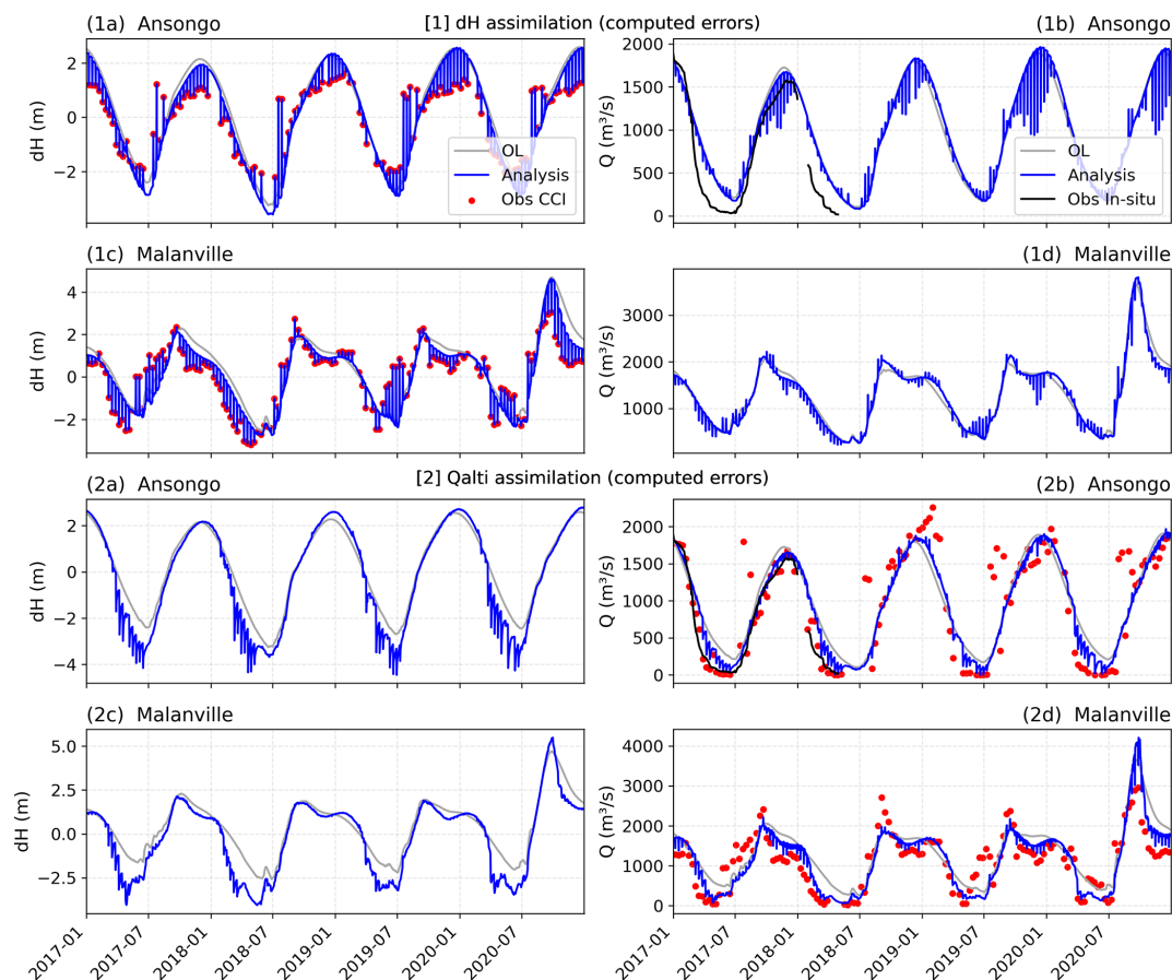
Figure 7. Comparison of water surface elevation ( dH ) and altimetry-based discharge ( Q_{\text{alti}} ) assimilation with computed errors for Ansongo and Malanville stations (2017–2020), within MGB-HYFAA. Panel (1a–d): dH assimilation (computed errors) showing time series of dH (1a, 1c) and discharge ( Q ) (1b, 1d) for Ansongo and Malanville. Panel (2a–d): Q_{\text{alti}} assimilation (computed errors) showing time series of dH (2a, 2c) and discharge ( Q ) (2b, 2d) for the same stations. Obs CCI represents water surface elevation (WSE) from satellite altimetry in panels (1a, 1c) and altimetry-derived discharge in panels (2b, 2d).
