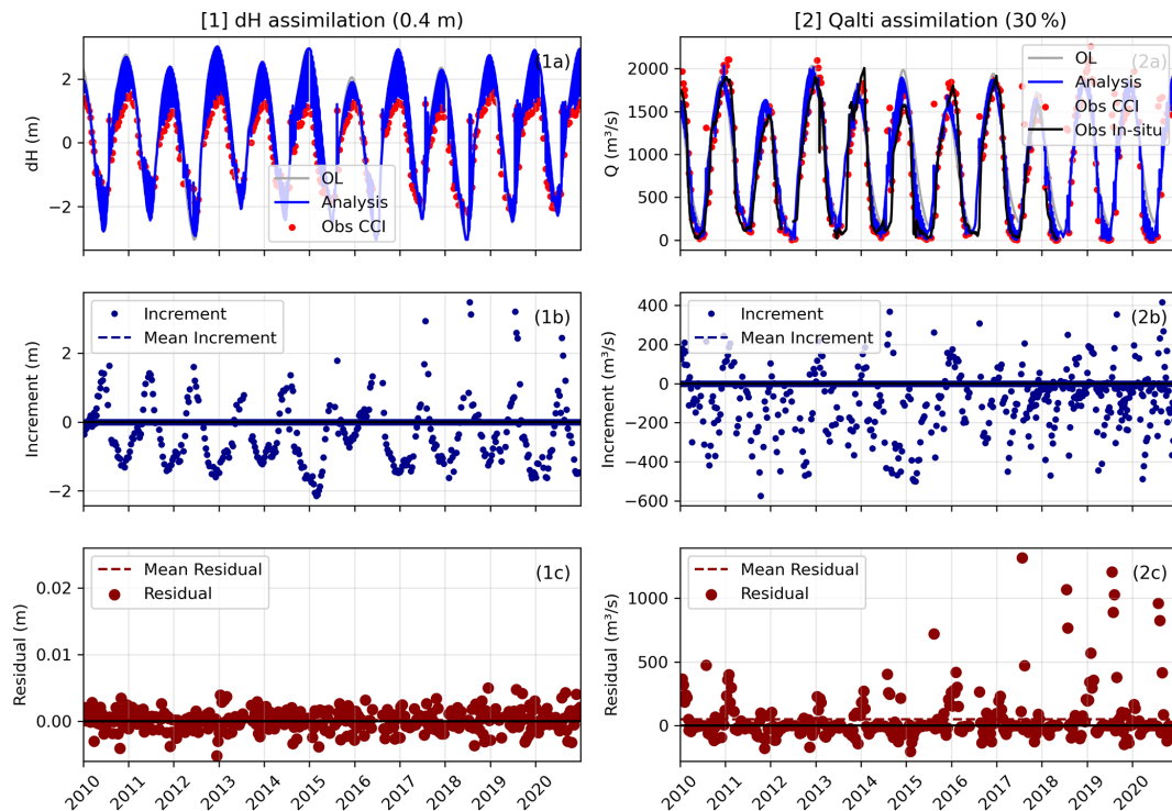
Figure 9. Comparison of dH and Q assimilation at Ansongo, Niger, over the 2010–2020 period, within MGB-HYFAA: Top panels show time series of (a) dH assimilation with 0.4 m uncertainty and (b) Q_{\text{alti}} assimilation with 30 % uncertainty, with open-loop, analysis, and observed data. The middle and lower panels show the corresponding innovation and residuals, with the mean innovation and residuals represented by dashed lines, illustrating the model's performance and adjustments after assimilation.
