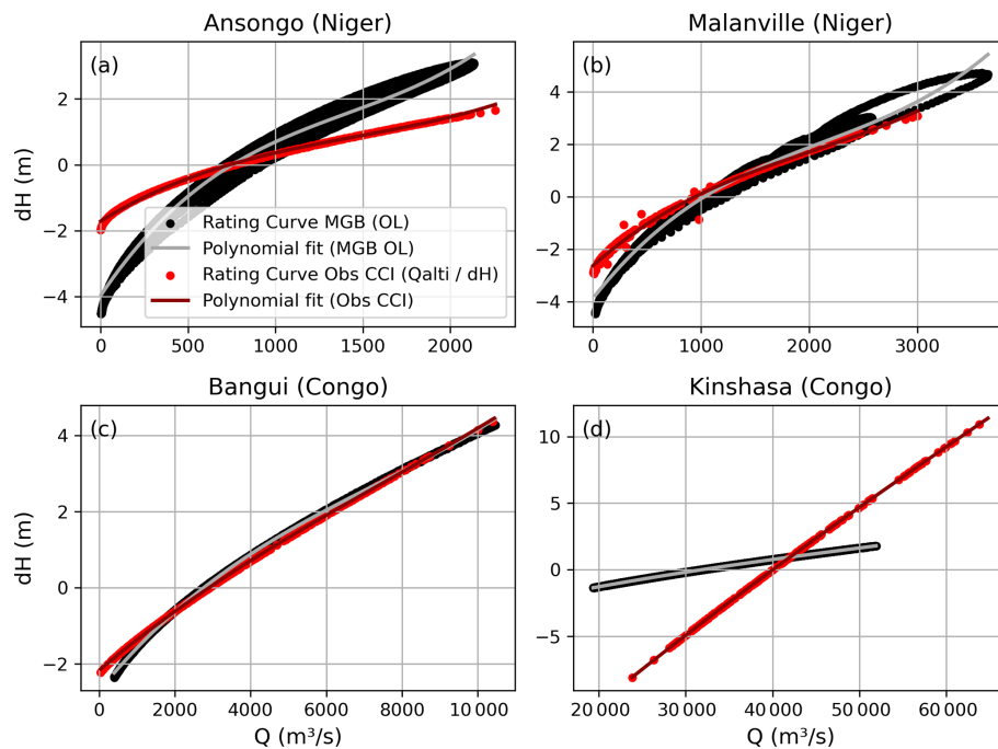
Figure 8. Rating curves from MGB (Open-Loop) vs. Obs CCI ( dH , Q_{\text{alti}} ) at (a) Ansongo and (b) Malanville stations in the Niger basin, and at (c) Bangui and (d) Kinshasa stations in the Congo basin.
