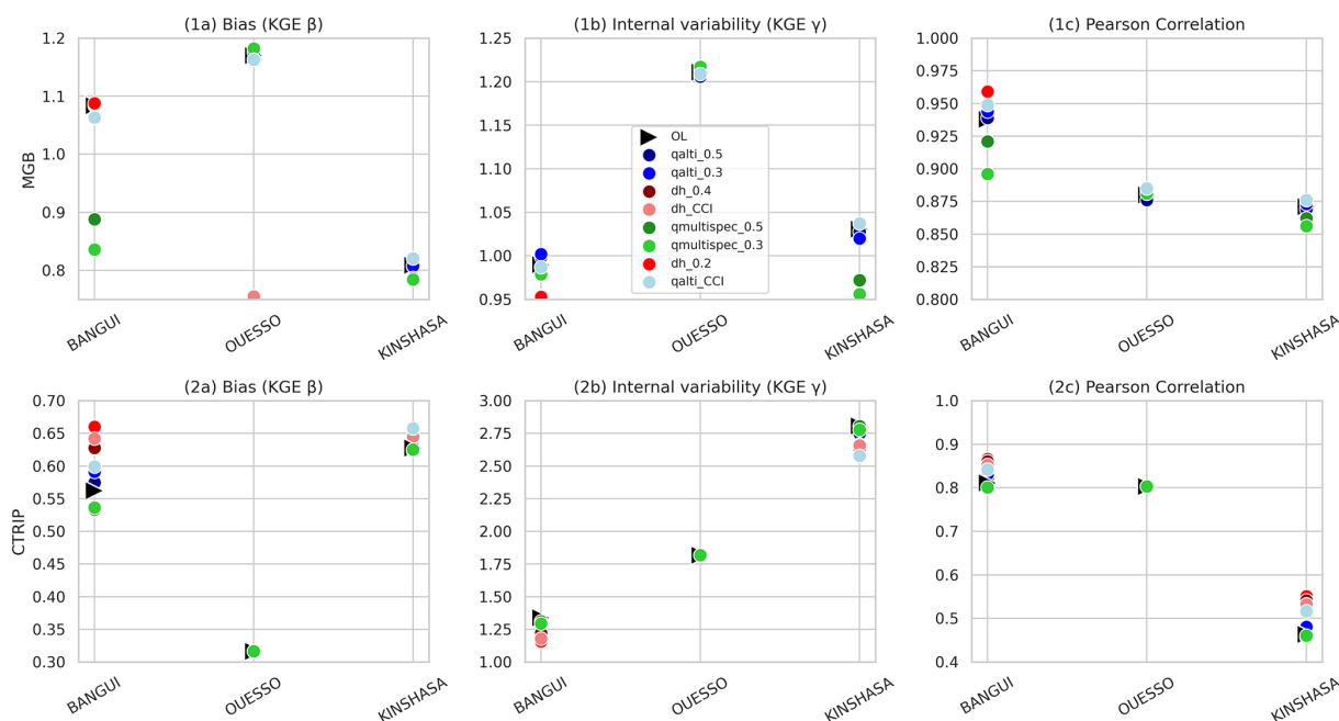
Figure 14. Comparison of bias (KGE \beta ), internal variability (KGE \gamma ), and Pearson correlation for different assimilation experiments in MGB (first line) and CTRIP (second line) models: daily scores at Ouesso, Bangui, and Kinshasa stations.
