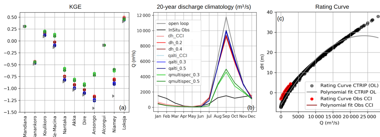
Figure 11. Panel (a) presents the Kling-Gupta Efficiency (KGE) performance results from CTRIP for each assimilation experiment (colored markers) at 11 stations in the Niger Basin, with Open-Loop (OL) performance shown as grey triangles for reference. Panel (b) displays the corresponding discharge climatology at Niamey, comparing observed discharge (black) with Open-Loop simulations from CTRIP (grey) and different assimilation experiments (colored), illustrating seasonal variations in modeled and observed discharge. Panel (c) shows the rating curve at Niamey from CTRIP Open-Loop (black), compared to Obs CCI (dH, Q_{\text{alti}} ) (red).
