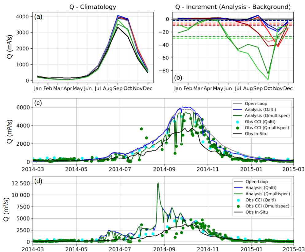
Figure 13. (a, b) MGB model results at Koulikoro for different experiments (dH in shades of red, Q_{\text{alti}} in shades of blue, Q_{\text{multispec}} in shades of green); (a) Discharge climatologies, with in-situ observations in black. (b) Increment (Analysis minus Background) shows differences after assimilation, with mean increments indicated by dashed lines. (c, d) Example of assimilation results over a year (2014) for Q_{\text{alti}} (blue) vs. Q_{\text{multispec}} (green) at Koulikoro within MGB (c) and CTRIP (d), both CCI products assimilated at 30 % uncertainty.
