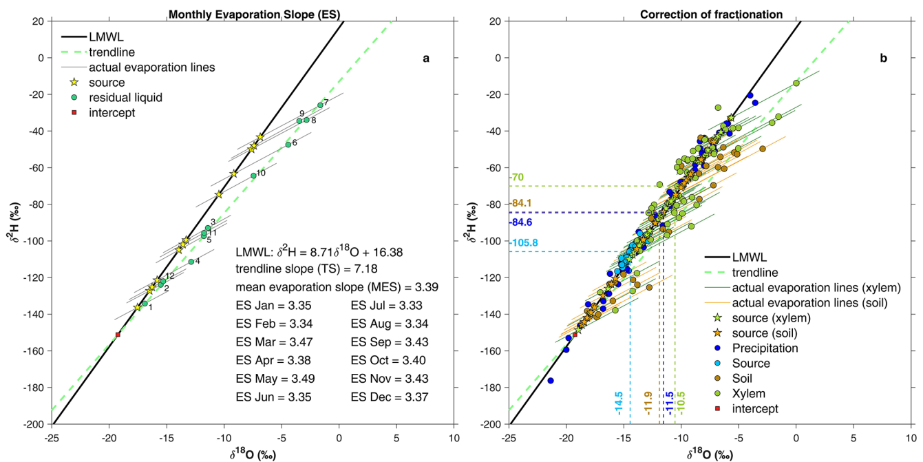
Figure 6. (a) Results of the monthly evaporation slopes (ES) obtained by applying the Craig and Gordon (1965) model being implemented by Benettin et al. (2018). The monthly ES have been used to reproject the fractionated water samples on the local meteoric water line (LMWL). The numbers next to the residual liquid points indicate the month (1: January; 12: December); (b) Isotopic fractionation correction for fractionated (line-conditioned excess* < 0) plant/soil water samples. Precipitation and Source (SOU) water samples have been also reported. The median isotopic composition of each reservoir is indicated by the dashed lines.
