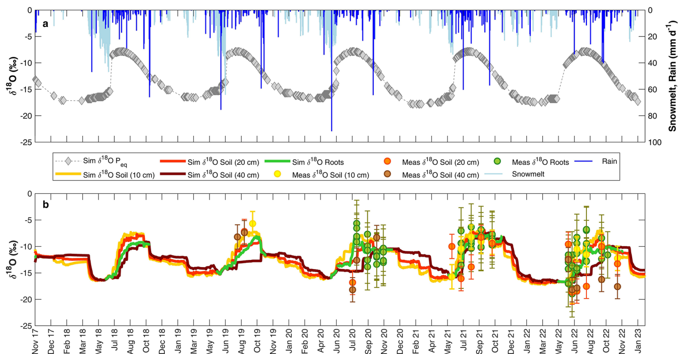
Figure 8. (a) Snowmelt, rain and isotopic composition of equivalent precipitation ( C_{P_{eq}} ). (b) Comparison of simulated soil/plant water isotopic composition at the three observation nodes (10, 20 and 40 cm) and measured soil/plant water isotopic composition. The maximum standard deviation (SD) values reported by Millar et al. (2022) are displayed as error bars.
