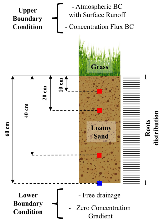
Figure 4. HYDRUS-1D setup. Red squares indicate observation points in which isotope and soil probes measurements are available. Blue square indicates an observation point in which measurements are not available.
