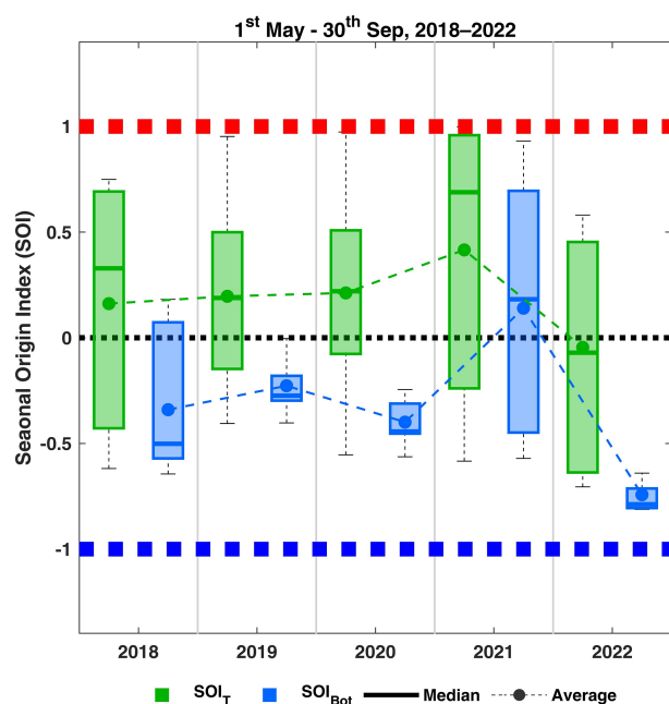
Figure 10. Seasonal Origin Index of transpiration ( \text{SOI}_T ) and bottom fluxes ( \text{SOI}_{\text{Bot}} ), simulated with HYDRUS-1D, during the growing seasons from 2018 to 2022.
