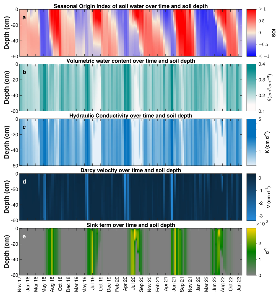
Figure 12. (a) Seasonal Origin Index (SOI). (b) Volumetric water content ( \theta ). (c) Hydraulic conductivity ( K ). (d) Darcy velocity ( V , the sign convention is positive upwards and negative downwards). (e) Sink term over time and soil depth. Please, note that only 138 print times from 1 November 2017 to 6 February 2023 with a 14 d time step are reported. In panel (a) the red color indicates \text{SOI} > 0 (summer water is overrepresented in the soil water), while the blue color indicates \text{SOI} < 0 (winter water is overrepresented in the soil water). All the variables over time and soil depth have been simulated with HYDRUS-1D.
