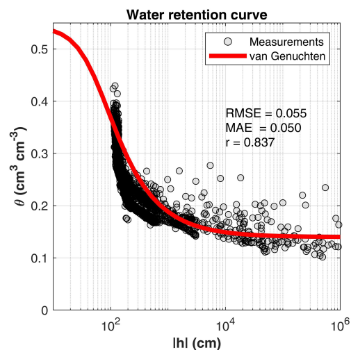
Figure 5. Volumetric water content ( \theta ) as a function of pressure head ( |h| ). Points represent measurements, while the solid red line denotes the optimized van Genuchten water retention function. Performance metrics (RMSE, MAE, and Pearson's correlation coefficient, r ) are reported.
