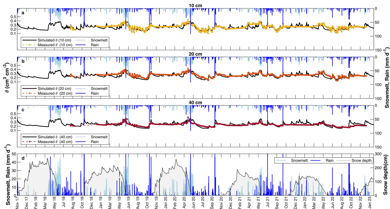
Figure 7. Measured (line with markers) and simulated (line) volumetric water content at (a) 10 cm, (b) 20 cm and (c) 40 cm. Snowmelt and rain have been also indicated. (d) Snow depth, snowmelt and rain. \theta indicates the volumetric water content.
