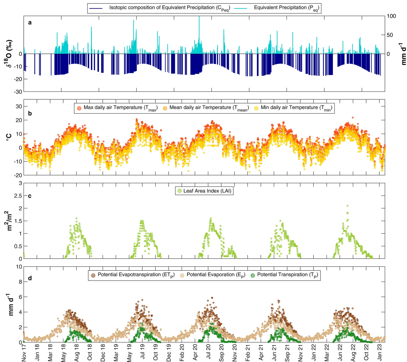
Figure 3. HYDRUS-1D input and related data obtained as described in Sect. 2.3–2.6. (a) Equivalent precipitation ( P_{eq} ) and corresponding isotopic composition ( C_{P_{eq}} ), (b) maximum ( T_{max} ), mean ( T_{mean} ) and minimum ( T_{min} ) daily air temperature, (c) Leaf Area Index (LAI), (d) Potential evapotranspiration ( ET_p ) computed with HSM, potential evaporation ( E_p ) and potential transpiration ( T_p ) obtained by applying the Beer’s law. Panels (a) and (d) show data of the time-variable boundary condition inputs used in HYDRUS-1D, while panels (b) and (c) present the intermediate variables used to compute the inputs in panel (d) .
