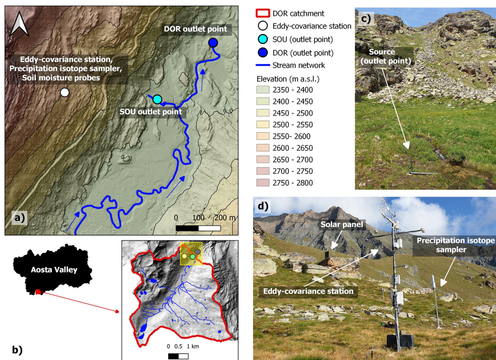
Figure 2. (a) Location of the study site within the Dora del Nivolet (DOR) catchment. Soil samples and lignified twigs/roots are collected nearby the eddy-covariance station where also volumetric water content and matric potential (10, 20, 40 cm depth) are measured. Blue arrows indicate the flow direction. (b) Geographical framework of the DOR catchment. (c) Photo (2 July 2019) of the monitored source (SOU). (d) Photo (23 August 2019) of the eddy-covariance station and of the precipitation isotope sampler. In the background it is possible to observe the solar panel that supplies the eddy-covariance station.
