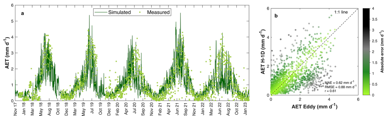
Figure 9. (a) Measured (AET Eddy) and simulated (AET H-1D) actual evapotranspiration. (b) AET H-1D versus AET Eddy.
