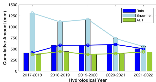
Figure 1. Cumulative values of rain, snowmelt, and actual evapotranspiration (AET) measurements (derived from the eddy-covariance station installed at the study-site) from hydrological years 2017–2018 to 2021–2022. An exception is made for the year 2017–2018, where measurements begin on 1 November 2017. Coloured bars represent yearly totals, and lines connect the top of each variable's bars across years to highlight temporal trends. Periods without available AET measurements were filled using linear interpolation prior to annual aggregation. Rain and snowmelt values shown in the figure are derived using the model by Ceperley et al. (2020), as described in Sect. 2.4.
