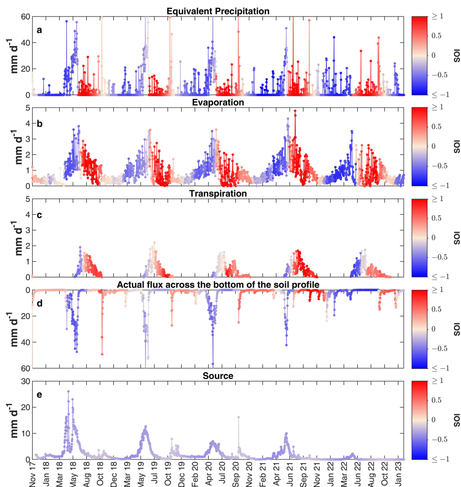
Figure 11. (a) Equivalent precipitation ( P_{eq} ). (b) Evaporation flux. (c) Transpiration flux. (d) Actual flux across the bottom of the soil profile. (e) Monitored spring (SOU) discharge. The red color indicates SOI > 0 (summer water is overrepresented in the flux), while the blue color indicates SOI < 0 (winter water is overrepresented in the flux). In panel (a) equivalent precipitation and the isotopic composition of equivalent precipitation ( C_{P_{eq}} ), from which the SOI has been calculated, are obtained with the Ceperley et al. (2020) model. In panels (b), (c) and (d) the fluxes and their isotopic composition, used to retrieve the SOI, are simulated by using HYDRUS-1D. In panel (e) the SOI isotopic composition is derived from measurements: in order to have a continuous isotopic composition (and consequently continuous SOI) at all time-steps we fit a sine function on data as described in von Freyberg et al. (2018).
