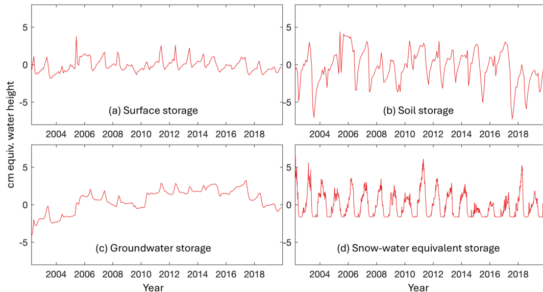
Figure 5. Cumulative HGS-based anomalies for (a) surface water storage, (b) soil moisture storage, and (c) groundwater storage, centred around the mean of the GRACE/GRACE-FO baseline period (January 2004–December 2009). (d) Snow-water equivalent storage is presented as an anomaly with respect to the same baseline but is not cumulated over the availability period.
