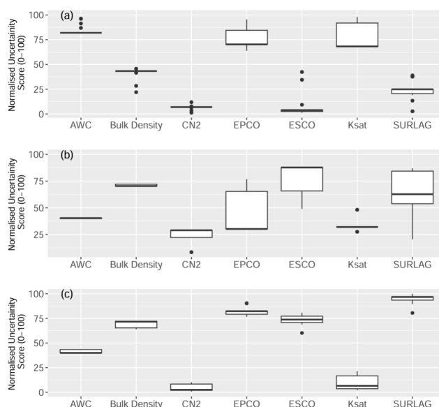
Figure 10. Parameter uncertainty estimate derived from DEoptim calibration iterations for (a) streamflow only, (b) soil-moisture only and, (c) multi-objective calibration. The height of the boxplot demonstrates the range of different values the parameters took while yielding acceptable model performance. The values are calculated using the normalized uncertainty score from Kumar and Merwade (2009), where 0 and 100 represent the minimum and maximum parameter value as defined by the normalized calibration range.
