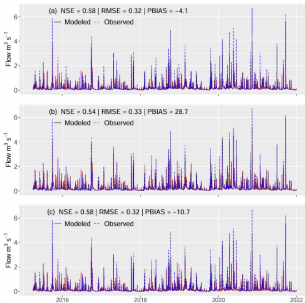
Figure A3. Full time series of model streamflow prediction performance calibration period (a) streamflow only (SF) calibration (b) soil-moisture only (DSM) calibration (c) multi-objective (MO) calibration.
