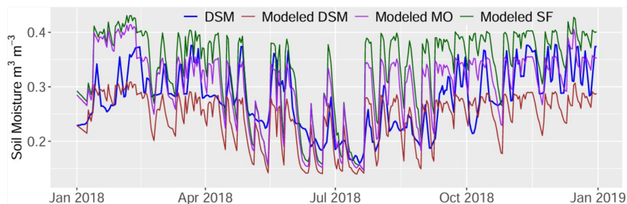
Figure A2. Time series of modeled surface soil-moisture (50 mm) from the three calibration approaches and DSM data; calibrated on DSM data (Modeled DSM), Multi-objective calibration using DSM data and streamflow (Modeled MO), calibrated on streamflow (Modeled SF).
