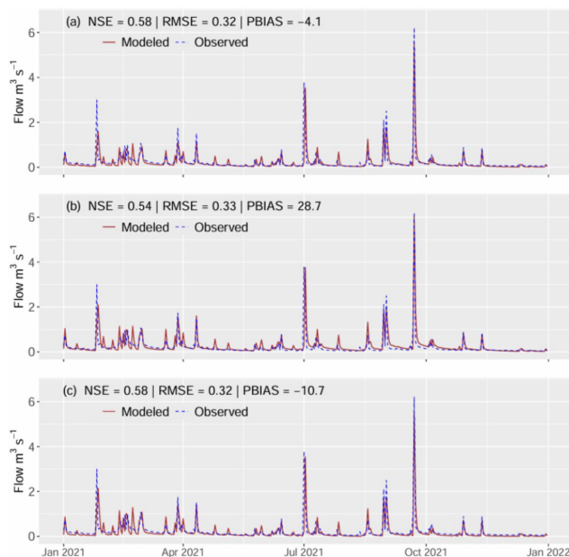
Figure 4. Model streamflow prediction performance calibration period (a) streamflow only (SF) calibration (b) soil-moisture only (DSM) calibration (c) multi-objective (MO) calibration (see Fig. A3 for the complete time series).
