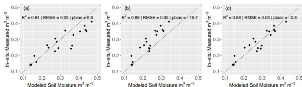
Figure 6. Soil-moisture estimation performance of the three models in the evaluation period at field-scale against field-scale average soil-moisture estimate from in-situ measurements; (a) streamflow only (SF) calibration (b) soil-moisture only (DSM) calibration (c) multi-objective (MO) calibration.
