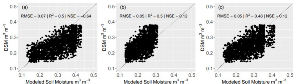
Figure 5. Model soil-moisture estimation performance during the calibration period compared against downscaled and bias corrected soil-moisture data calibrated on (a) streamflow only (SF) calibration (b) soil-moisture only (DSM) calibration (c) multi-objective (MO) calibration.
