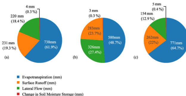
Figure 8. Model water balance estimation (a) streamflow only (SF) calibration (b) soil-moisture only (DSM) calibration (c) multi-objective (MO) calibration.
