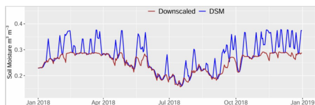
Figure 3. Time series of downscaled (mlrhm product) and downscaled-bias-corrected soil-moisture (DSM) at the watershed-scale. Data from only one year are shown for clarity.
