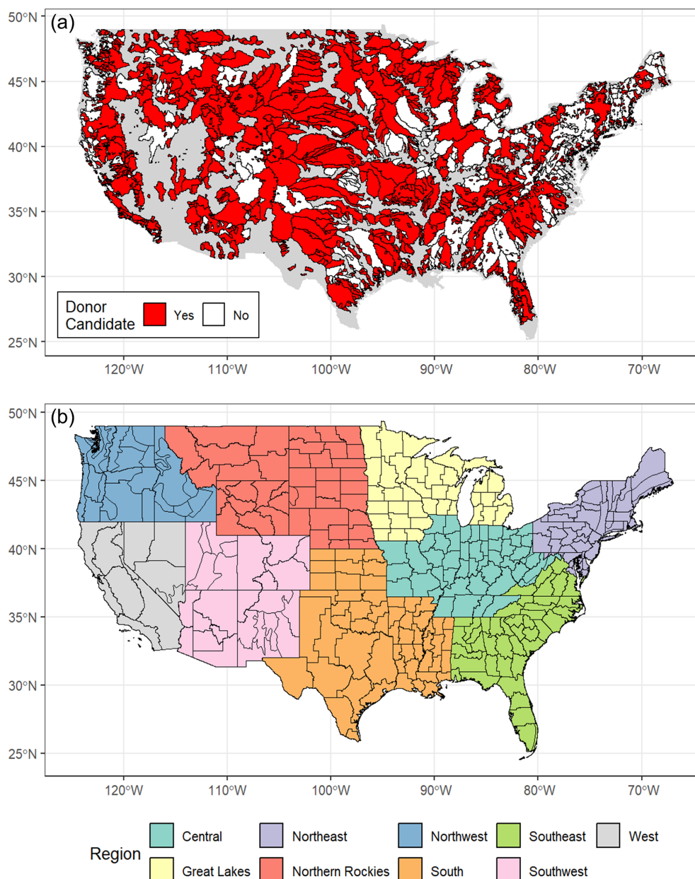
Figure 1. Panel (a) shows the 3198 basins in the conterminous United States which comprise the study area. Red basins indicate the 1900 filtered basins with Kappa > 0.4 used as candidate donors. The filtering process is described in Sect. 2.4.1. For ease of reference in describing results, we divided the CONUS into nine geographic regions (panel b), which shows regional naming conventions.
