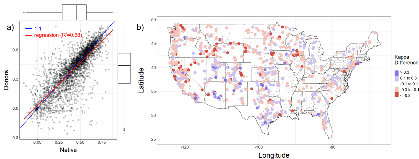
Figure 7. A comparison between donor-based model accuracy and at-site model accuracy at 3198 sites in the CONUS. Panel (a) is a scatterplot showing the relationship between at-site and donor-based models and corresponding boxplots showing model distributions, and panel (b) is a map showing the differences between donor-based and at-site model Kappa values. Sites with less than a 0.1 absolute difference are represented with small grey points.
