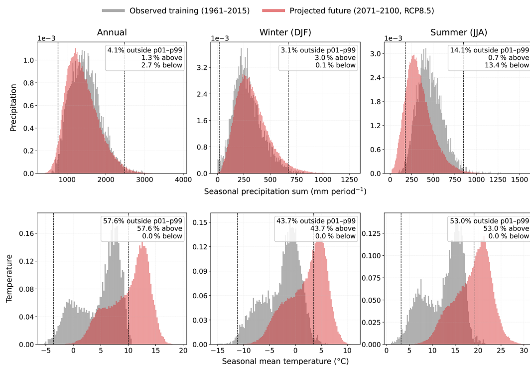
Figure A2. Comparison of seasonal atmospheric forcing distributions between the observational LSTM training data and late-century CH2018 projections. Histograms show catchment–season–year summaries for the 96 observational training catchments during 1961–2015 and for the 307 projection catchments during 2071–2100 under RCP8.5. Columns correspond to annual, winter (DJF), and summer (JJA) values; rows show seasonal precipitation sums and seasonal mean temperature. Dashed vertical lines indicate the 1st and 99th percentiles of the observational training distribution, and annotations report the percentage of future projected values outside this percentile range.
