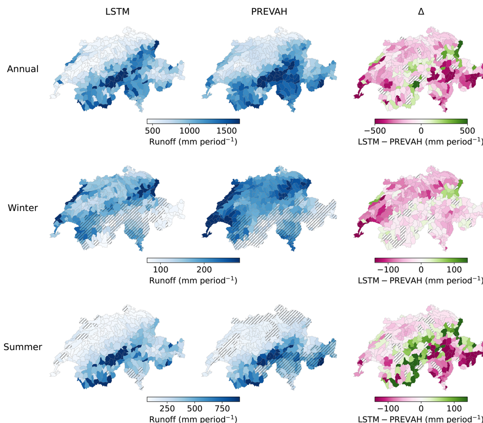
Figure 5. Spatial distribution of mean seasonal runoff for the RCP8.5 historical baseline (1991–2020). Panels are arranged in a 3 \times 3 grid by season (rows: Annual, Winter [DJF], Summer [JJA]) and by model output (columns: LSTM median, PREVAH median, \Delta = \text{LSTM} - \text{PREVAH} ). Each map shows the median over 14 ensemble chains of the 30-year mean seasonal total. Colorbars under columns 1–2 span the 5th–95th percentile of median runoff ( \text{mm period}^{-1} ), and under column 3 a diverging scale for \Delta ( \text{mm period}^{-1} ). Hatch marks on the LSTM and PREVAH maps denote catchments whose coefficient of variation of the long-term mean seasonal runoff across ensemble chains exceeds 10 %. Hatch marks in column 3 flag catchments where a robust signal-to-noise ratio is < 1 , with \text{SNR} = |\text{median}(r_c)|/\text{MAD}(r_c) and r_c = 2(L - P)/(|L| + |P| + \varepsilon) , where L and P denote the runoff simulated by the LSTM and PREVAH models, respectively. This indicates that the median model difference is small or not robust relative to inter-chain variability.
