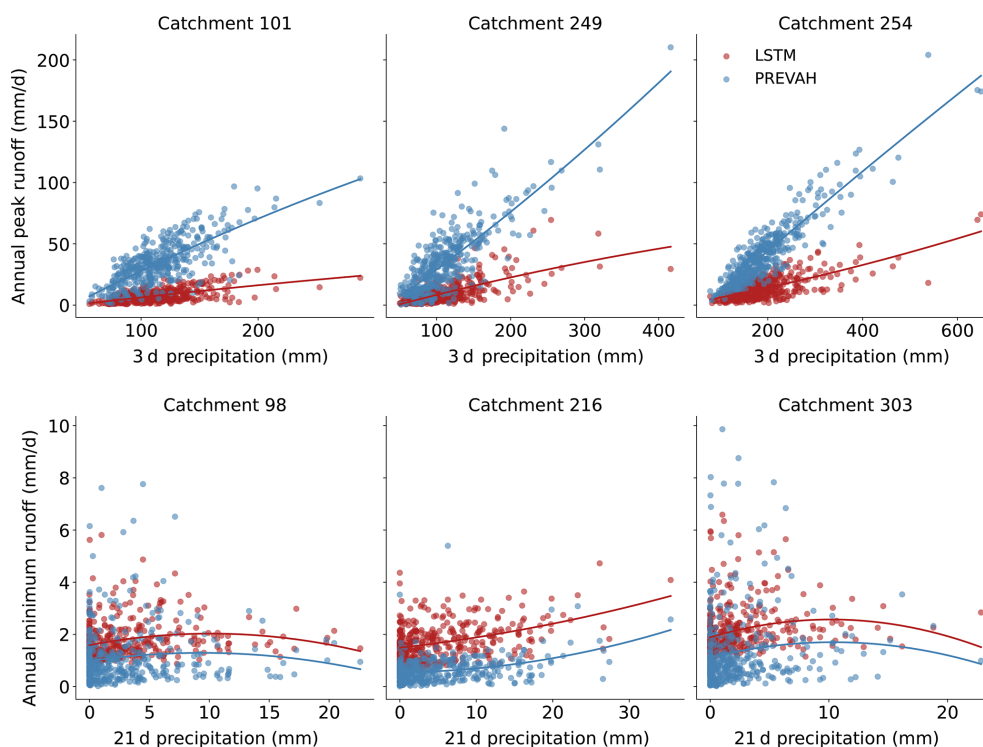
Figure 10. Catchment-level relationships between antecedent precipitation and extreme runoff under RCP8.5 for 2071–2099. Top row: annual maxima (red: LSTM, blue: PREVAH) at the date of maximum 3 d rolling precipitation versus that precipitation sum, for the three catchments with the largest negative LSTM–PREVAH maxima differences (IDs 101, 249, 254). Bottom row: annual minima runoff at the date of minimum 21 d rolling precipitation versus that precipitation sum, for the three catchments with the largest positive LSTM–PREVAH minima differences (IDs 98, 216, 303). Each point is one chain–year event; quadratic regression curves are overlaid.
