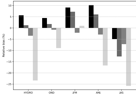
(b) Relative bias between AROME and Météo-France stations
