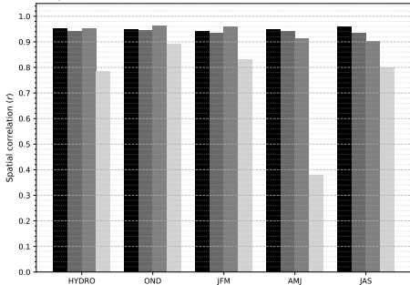
(a) Spatial correlation between AROME and Météo-France stations
