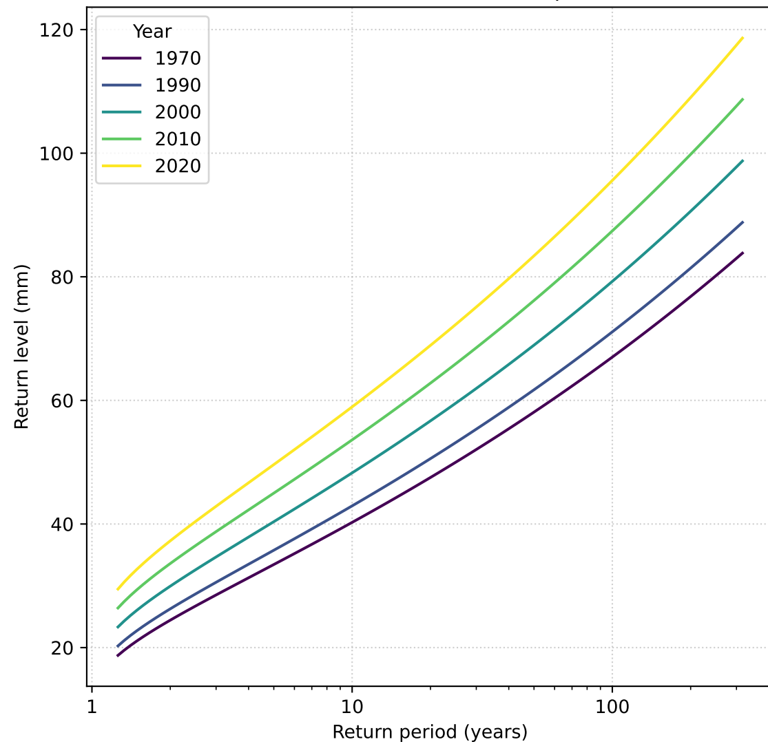
C: Associated return level plot
