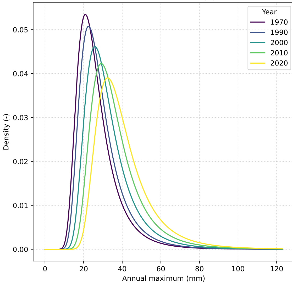
B: Associated GEV density plot
