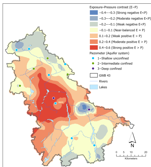
Figure 8. Spatial contrast between normalised Exposure ( E ) and Pressure ( P ) in GWB 43. Positive values indicate areas where E exceeds P , negative values indicate areas where P exceeds E , and values between -0.1 and 0.1 represent a balanced contrast. The E - P classes provide a descriptive comparison of the relative mapped component magnitudes and should not be interpreted as causal attribution.
