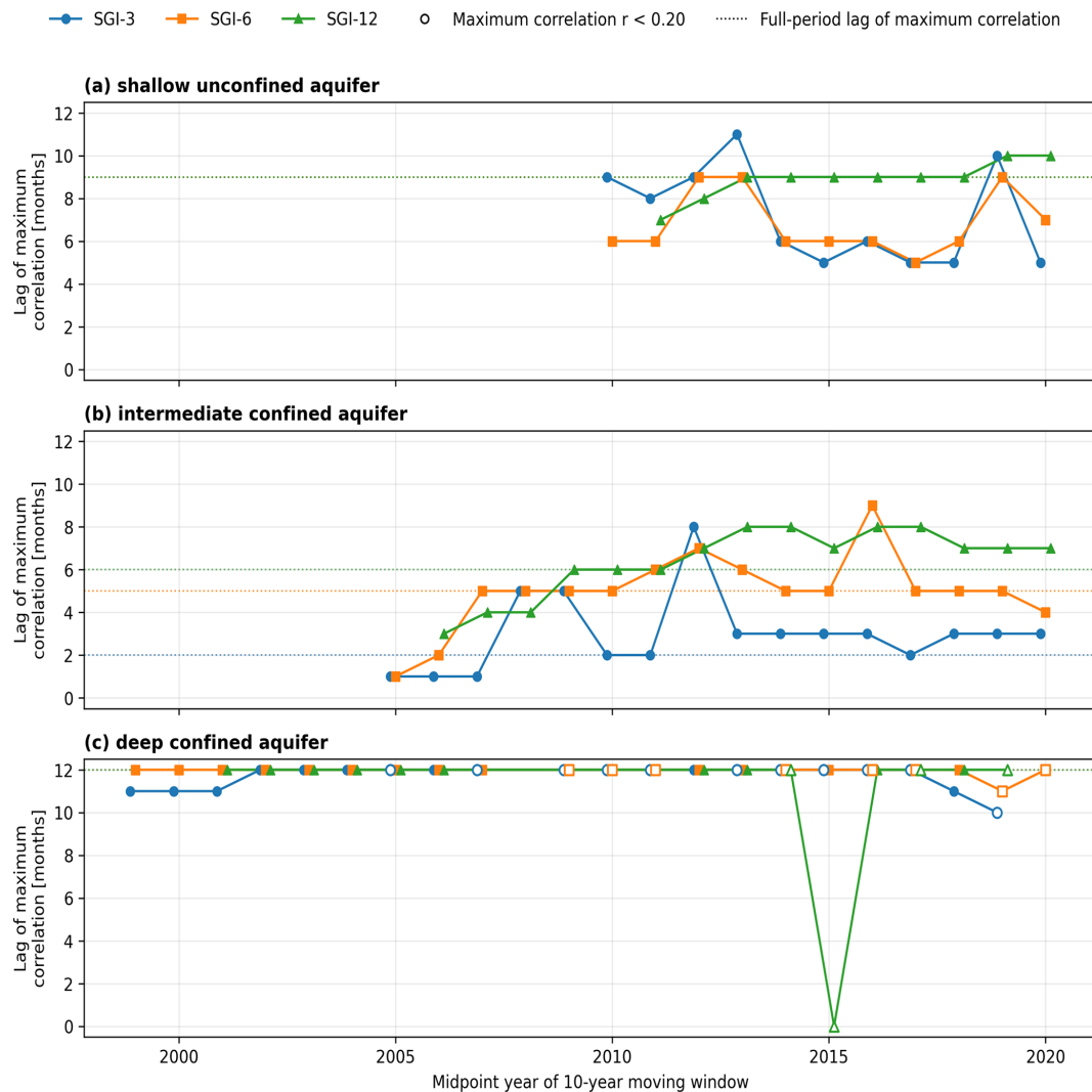
Figure C1. Temporal stability of the lag associated with the maximum SPI-SGI correlation in the three aquifer systems. The panels show results for (a) the shallow unconfined aquifer, (b) the intermediate confined aquifer, and (c) the deep confined aquifer, calculated using 10-year moving windows shifted forward by 1 year. Symbols indicate the lag of the maximum Pearson correlation for SGI-3, SGI-6, and SGI-12. Open symbols denote cases in which the maximum correlation was weak ( r < 0.20 ). Horizontal dotted lines indicate the full-period lag of maximum correlation for each SGI aggregation scale. Values reaching the upper tested limit of 12 months indicate that the actual response delay may exceed the analysed lag range.
