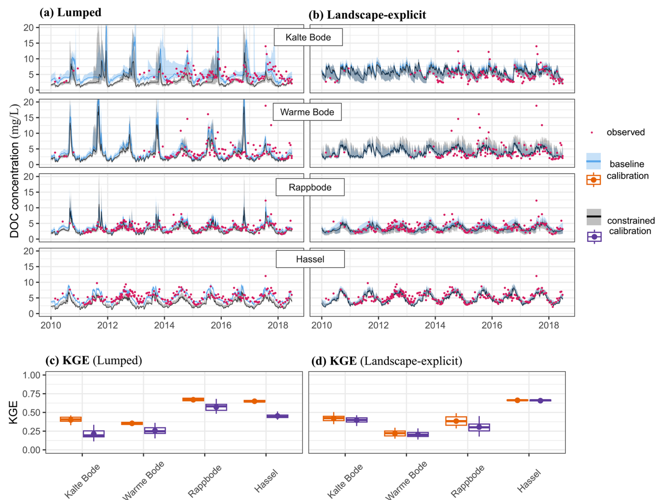
Figure 5. (a, b) Observed and simulated stream DOC concentration from the lumped and the landscape-explicit model structures under the baseline (blue) and constrained (grey) calibrations, along with the model performance (c, d) for both calibration and validation periods together instead of separating the results by calibration and validation periods. Simulated results were taken from 30 behavioural DOC simulations. The dots in the boxplots are the means.
