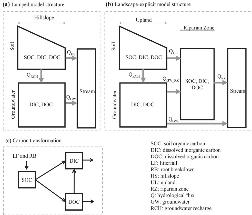
Figure 1. Conceptual representation of (a) the lumped model structure, (b) the landscape-explicit model structure, and (c) the carbon transformation among different carbon pools.
