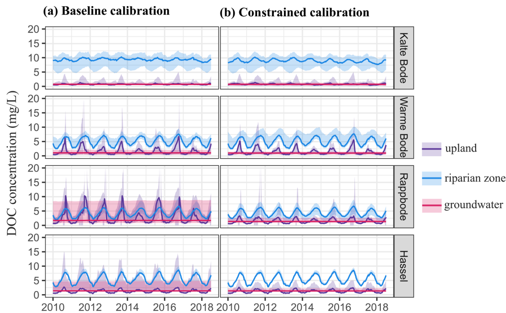
Figure 7. Internal DOC concentrations in different landscape units from the landscape-explicit model structures under (a) the baseline and (b) constrained calibrations.
