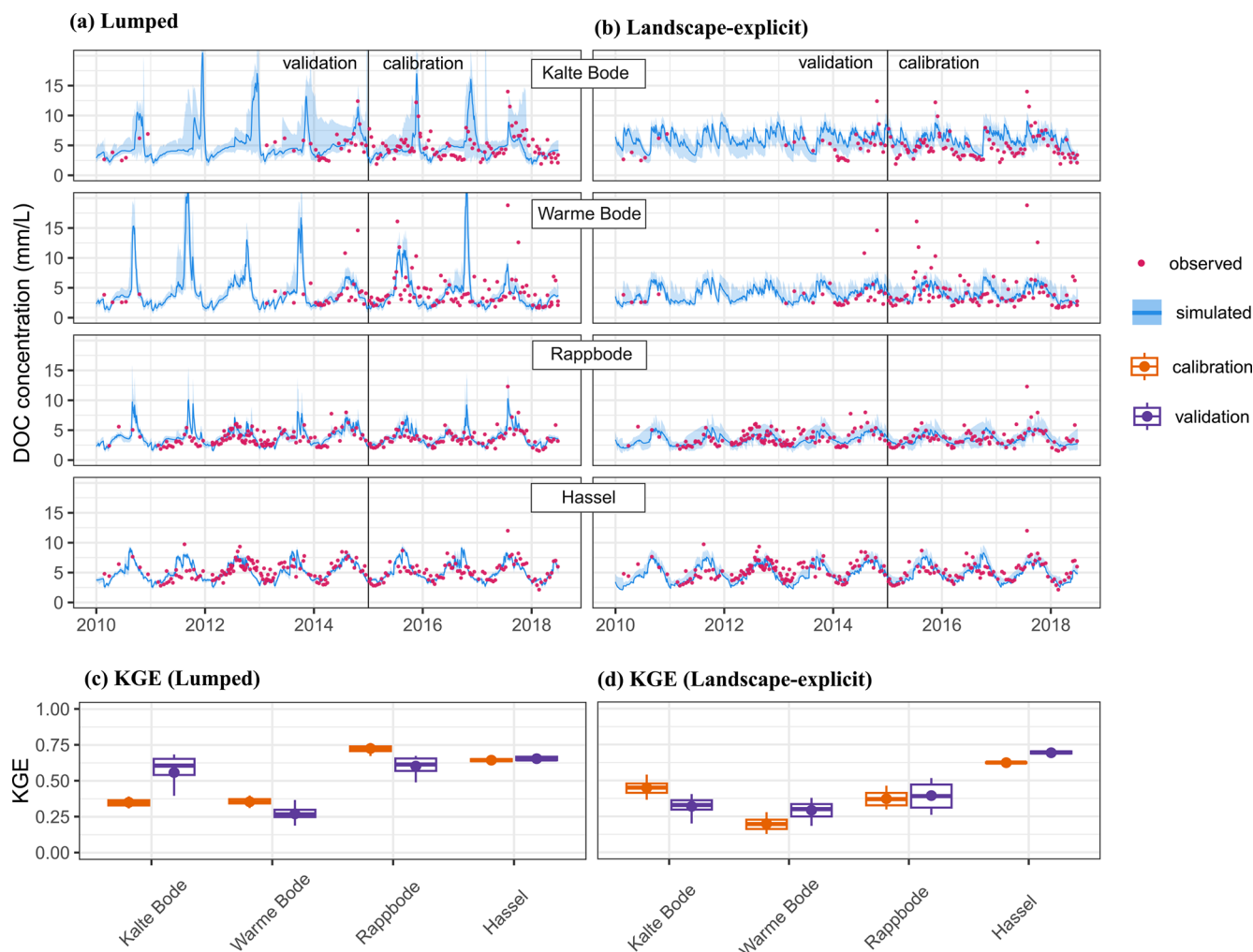
Figure 4. (a, b) Time series of observed and simulated stream DOC concentrations and (c, d) the model performance of 30 behavioural DOC simulations from (a, c) the lumped and (b, d) the landscape-explicit model structures during the calibration and validation of the baseline calibration. The solid lines and shaded areas (in blue) represent the medians and simulated ranges of these behavioural models. The dots in the boxplots are the means.
