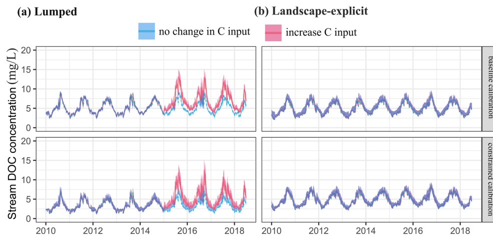
Figure 8. Simulated stream DOC concentrations in the Hassel catchment with increasing C input by 5 \text{ kg ha}^{-1} for the period 2015–2018 (a) in the hillslope of the lumped model structure, and (b) in the upland of the landscape-explicit model structure.
