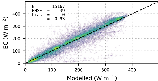
Daily SW Irradiance
