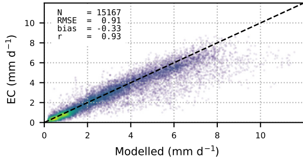
FAO56 \text{ET}_r
