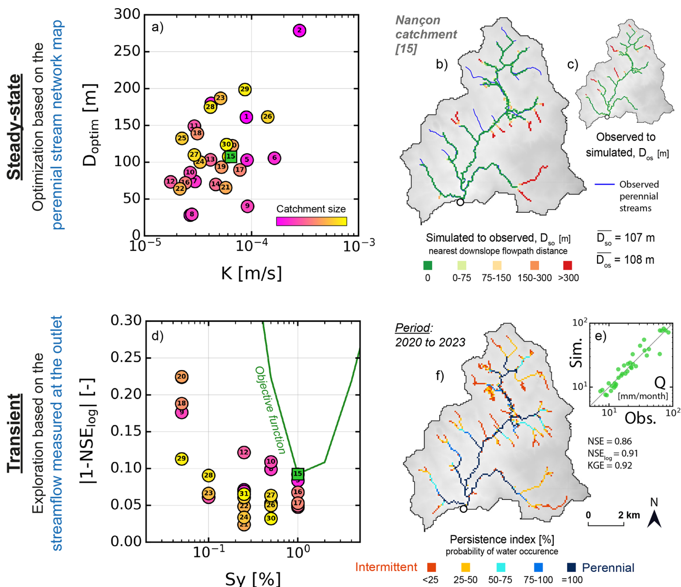
Figure 5. Calibration results for the estimation of hydraulic conductivity K and specific yield Sy for 31 catchments: (a) The best value of hydraulic conductivity K versus D_{\text{optim}} . The color bar represents relative catchment size. The green square highlights the Nançon catchment. (b) Simulated hydrographic network showing the distance D_{SO} from simulated seepage pixels to the nearest downslope observed stream network. (c) Similar representation for D_{OS} . (d) The best value of specific yield Sy obtained for each catchment versus the associated |1 - NSE_{\log}| criterion. The green line represents the objective function of the Nançon catchment. (e) Comparison of observed and simulated specific streamflow at the catchment outlet Q . The black line indicates the 1 : 1 relationship. (f) Representation of the persistence index of the simulated results, showing maximum (orange lines, highly intermittent) and minimum (dark blue lines, perennial) extents of the simulated stream network.
