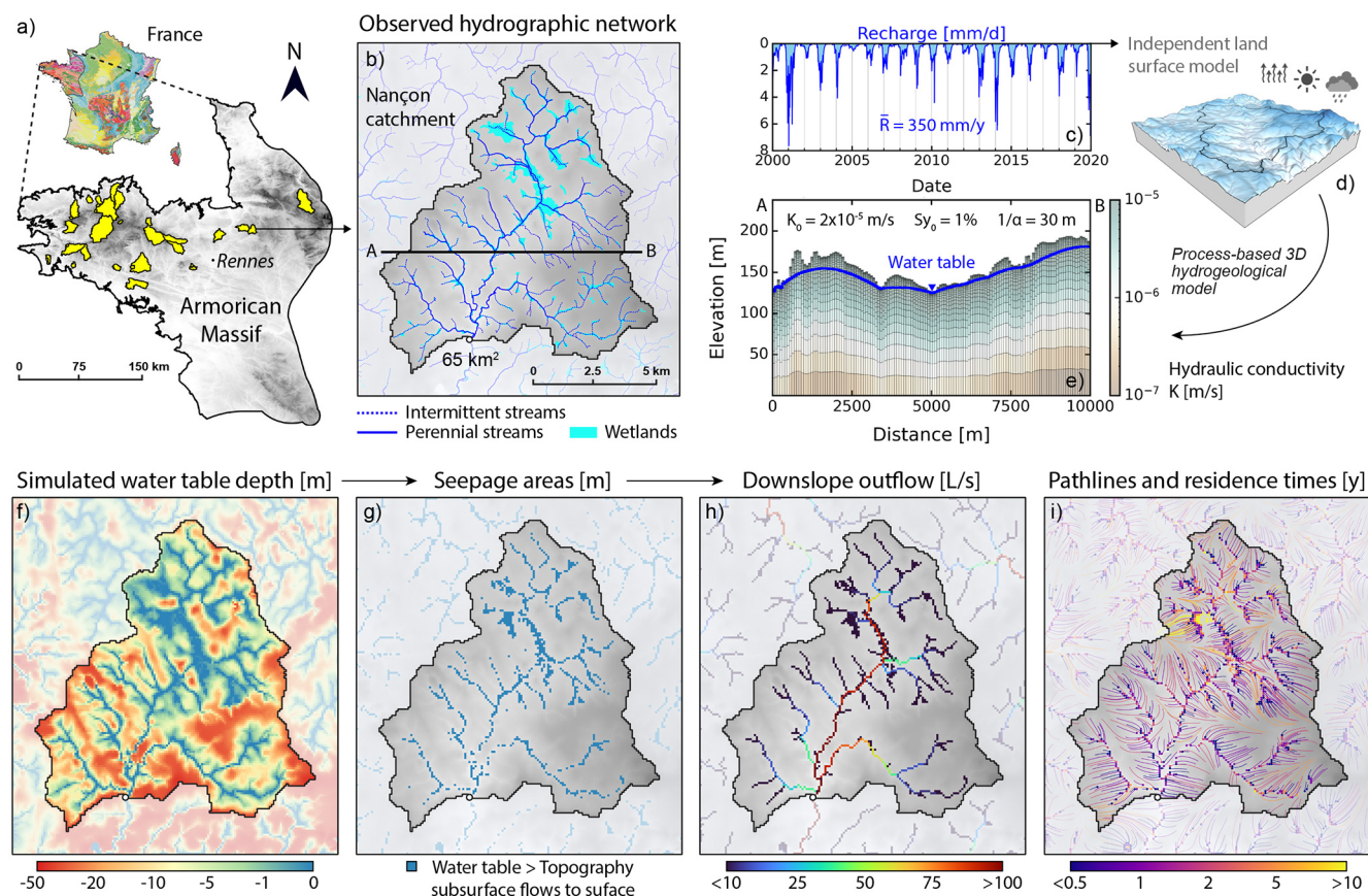
Figure 2. HydroModPy modeling steps illustrated for the Nançon catchment, Brittany (France). (a) Extraction of the watershed from a regional DEM, located to the west of the Geological Map of France. (b) Clip data based on the watershed extent. (c) Recharge time series provided from an independent land surface model. (d) 3D diagram illustrating the model conceptualization and parameterization based on data available and assumptions. (e) The cross-section (A–B) illustrates the vertical grid discretization and the resulting water table. The parameters include an exponential decay 1/\alpha with depth from the maximum hydraulic conductivity K_0 and specific yield S_{y0} (%) in the first layer. (f–i) 2D map top-view visualization displaying spatial data and model results in steady state across the study area (left to right): water table depth, seepage areas, accumulated outflow, pathlines, and residence times.
