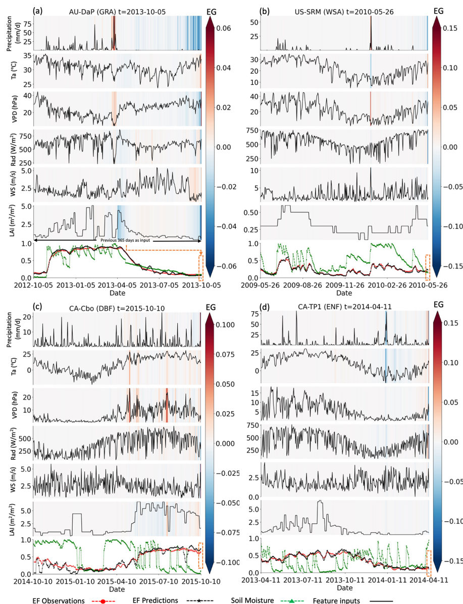
Figure 5. Examples of memory effects revealed by Expected Gradients. (a) A grassland site (AU-DaP, 5 October 2013). The LSTM model uses the previous 365 d of input data (from 5 October 2012 to 5 October 2013) to predict EF on 5 October 2013. Expected Gradients illustrate the contributions of antecedent climate variables, e.g., precipitation, air temperature, vapor pressure deficit (VPD), net radiation, and LAI, to the current EF prediction. During this long drydown event, precipitation around 5 April 2013 shows a positive contribution to EF. VPD and LAI also exhibit notable contributions. (b) A woody savanna site (US-SRM, 26 May 2010); (c) a deciduous broadleaf forest site (CA-Cbo, 10 October 2015); and (d) an evergreen needleleaf forest site (CA-TP1, 11 April 2014). Expected Gradient patterns across all sites are summarized in the subsequent figures.
