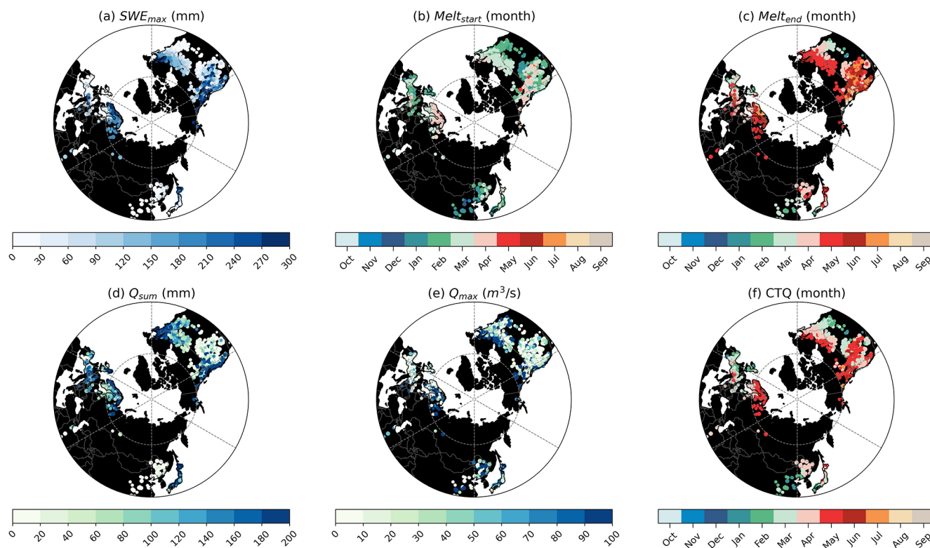
Figure 2. The spatial pattern of snow and runoff characteristics. (a) shows maximum snow water equivalent, (b) and (c) show the start and end timing of snowmelt. (d)–(e) present total runoff ( Q_{\text{sum}} ), peak flow ( Q_{\text{max}} ) and centroid timing of runoff (CTQ) during the snowmelt period, respectively. \text{Melt}_{\text{start}} , \text{Melt}_{\text{end}} , and CTQ are shown as the months instead of 'Day of Water Year' (DOY) for better interpretation of the results.
