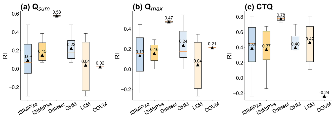
Figure 9. Assessment of model robustness in key SMR characteristics grouped by model categories and ISIMIP phase. (a)–(c) show results for Q_{sum} , Q_{max} , and CTQ, respectively. The orange line denotes the median, the black triangle indicates the mean, and the classifications of model types and ISIMIP phases follow Sect. 2.1.1.
