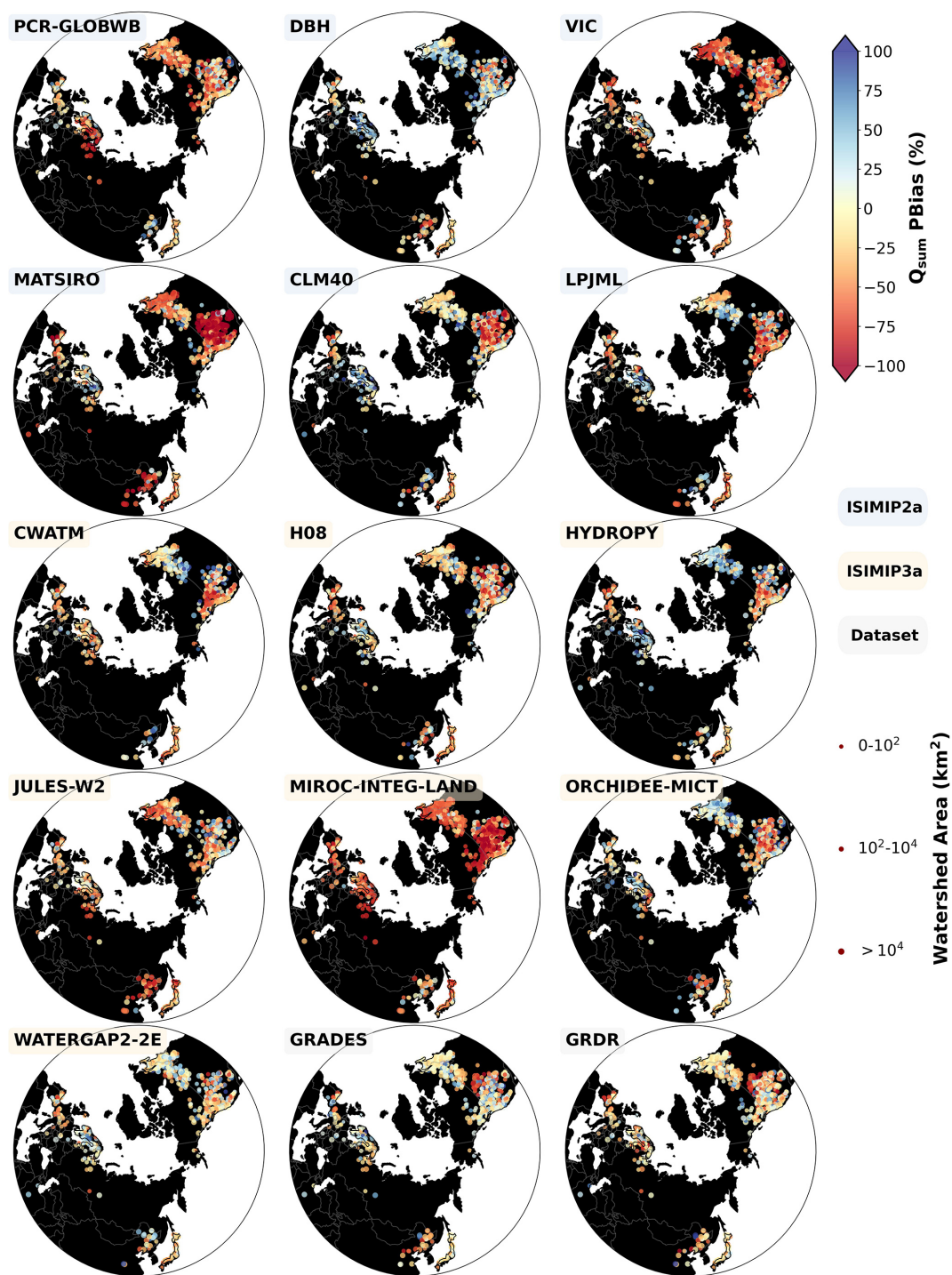
Figure A5. The percentage bias of total runoff ( Q_{sum} ) during the snowmelt period (unit: %). Colors indicate the degree of bias compared to observations: red represents underestimation, blue indicates overestimation, and yellow signifies well-matched total runoff. The point size is adjusted based on station density for better visualization and does not have physical significance. Colored boxes around model/dataset names denote three categories of data.
