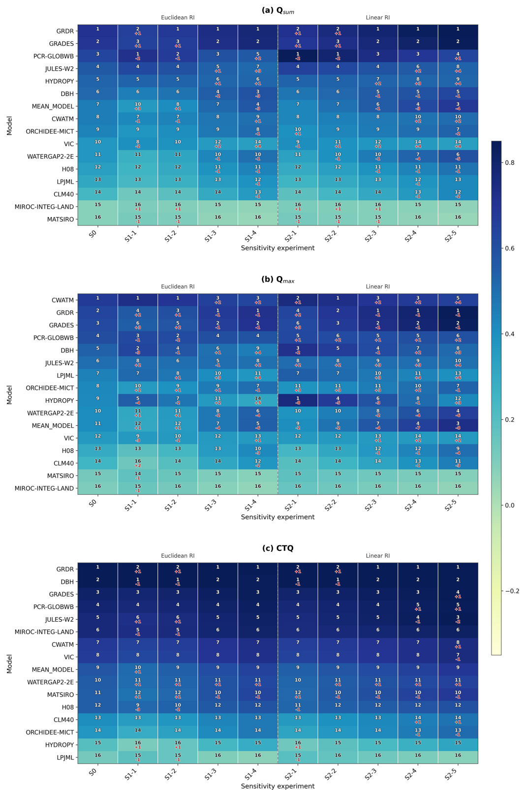
Figure A3. Sensitivity analysis of the Robustness Index (RI) formulation. Panels (a)–(c) present the sensitivity of model robustness rankings for Q_{sum} , Q_{max} , and CTQ, respectively. The sensitivity experiments include the baseline Euclidean-distance-based RI (S0), weighted Euclidean formulations (S1-1 to S1-4), and weighted linear formulations (S2-1 to S2-5). The color shading represents the RI value, and the number in each cell denotes the model rank under the corresponding experiment. Red numbers indicate rank changes relative to the baseline RI formulation.
