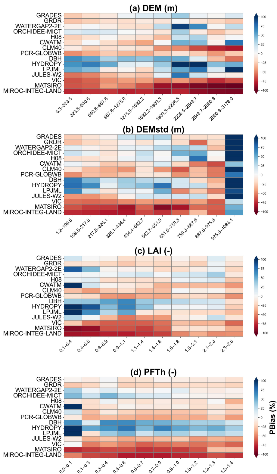
Figure A9. The bias in peak flow ( Q_{max} ) in the snowmelt period as a function of basin complexity factors. The value of each grid represents the median bias (color shading) within the corresponding range of DEM, DEMstd, LAI, and PFTth. The figures are ordered from top to bottom based on the proportion of biases within \pm 20\% .
