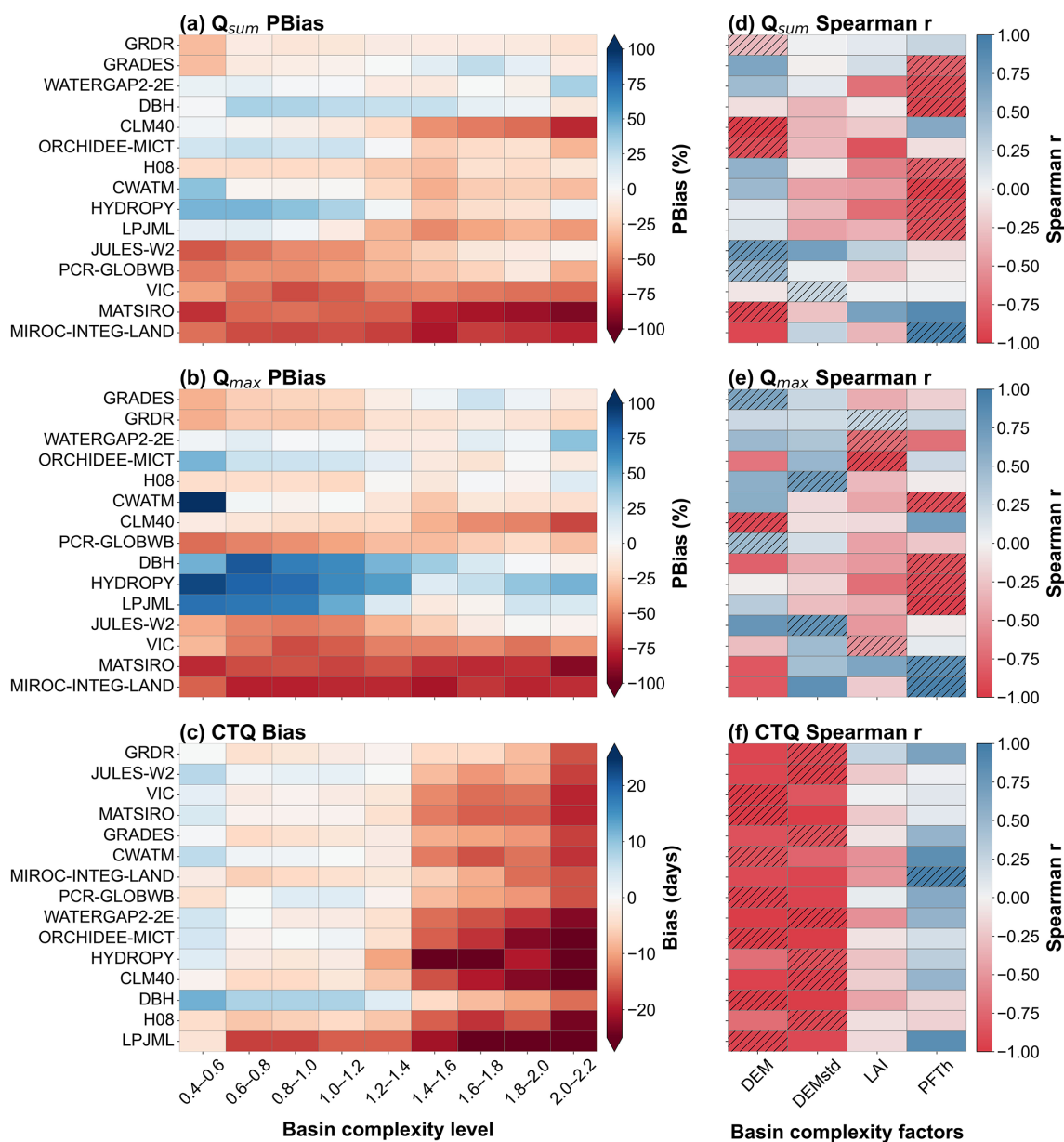
Figure 7. Influence of basin complexity on model simulations of key runoff characteristics. (a)–(c) show the variation in model performance as basin complexity increases, and (d)–(f) represent the Spearman correlation between model performance and individual basin complexity factors. A positive correlation indicates that model bias increases with increasing basin complexity, whereas a negative correlation indicates that model bias decreases as basin complexity increases. Shading indicates the basin complexity factor with the highest absolute Spearman correlation among the four factors.
