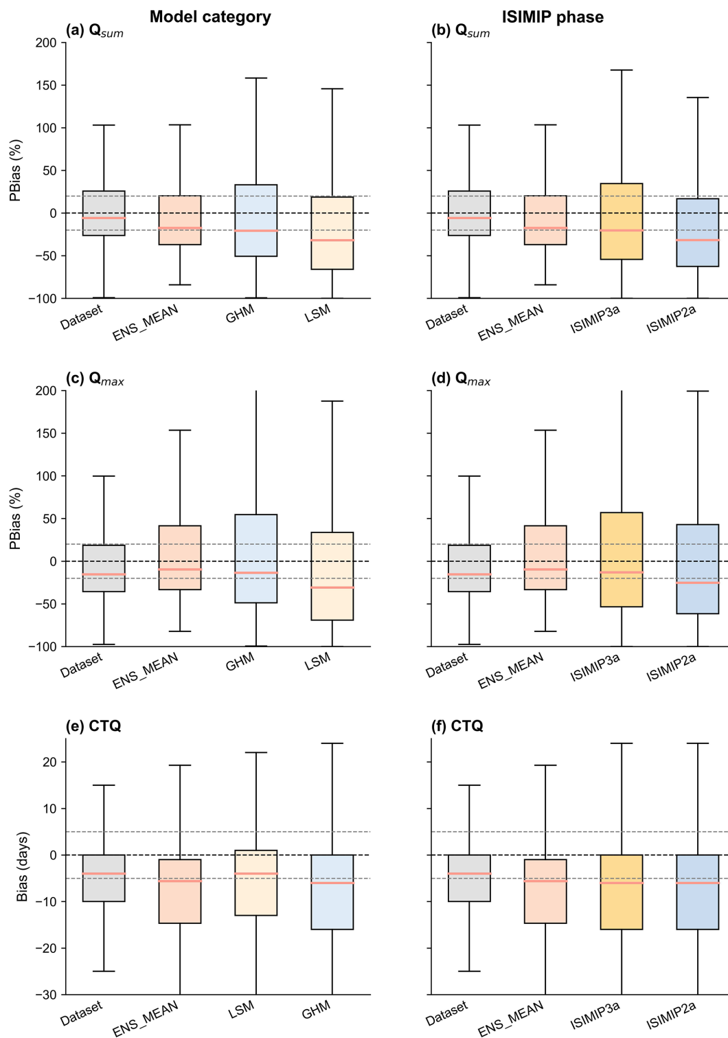
Figure 5. Evaluation of simulated runoff over 1979–2019 across 1455 catchments grouped by model category and ISIMIP phase. Panels (a), (c), (e) show the bias distributions grouped by model category, including global hydrological models (GHMs), land surface models (LSMs), observation-constrained runoff datasets (Dataset), and the ensemble mean of all individual models (ENS_MEAN). Panels (b), (d), (f) show the corresponding results grouped by ISIMIP phase. Rows represent the three snowmelt runoff characteristics: total runoff ( Q_{\text{sum}} ; a–b), peak flow ( Q_{\text{max}} ; c–d), and centroid timing of runoff (CTQ; e–f). The black dashed line indicates zero bias, and the gray dashed lines denote the acceptable ranges ( \pm 20\% for Q_{\text{sum}} and Q_{\text{max}} , and \pm 5 d for CTQ). Groups are ordered according to the proportion of basins falling within these acceptable ranges, with category-level rankings calculated from the average performance of individual models within each group.
