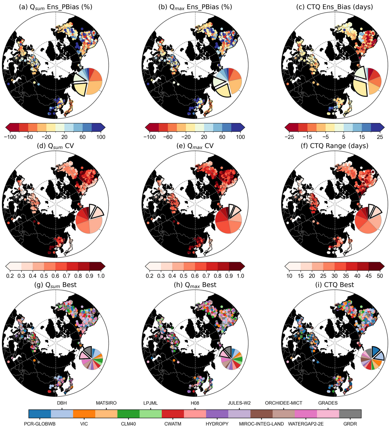
Figure 6. Bias, variability, and the best model for simulated SMR characteristics across different basins. (a)–(c) show the percent bias of Q_{sum} (%), percent bias of Q_{max} (%), and bias of CTQ (days), respectively, in the simulated SMR. (d)–(f) show inter-model variability represented by the coefficient of variation (CV) for Q_{sum} and Q_{max} , and inter-model range of CTQ (days). (g)–(i) show the model with the smallest bias in each basin for Q_{sum} , Q_{max} , and CTQ, respectively. The pie charts provide a summary of these patterns, with bold black outlines highlighting the proportion within \pm 20\% bias in (a)–(c), the two lowest variability levels in (d)–(f), and the top two models with the highest proportions in (g)–(i).
