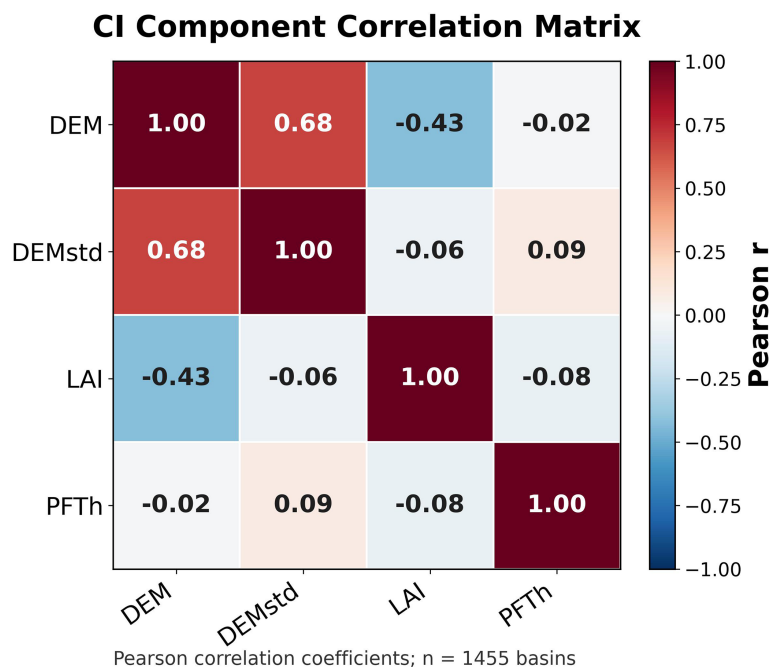
Figure A1. Pearson correlation matrix among the four components used to construct the basin complexity index. The value of each grid represents the Pearson correlation coefficients among the DEM, DEMstd, LAI, and PFTth.
