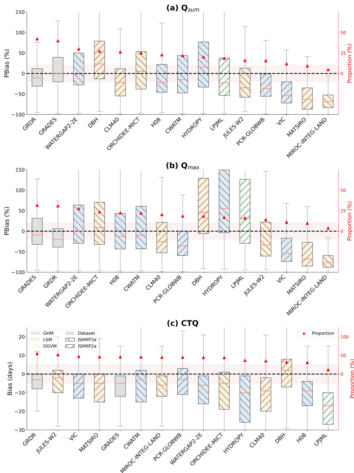
Figure 4. Evaluation of key SMR characteristics (averaged over 1979–2019) simulated by 15 models/datasets across 1455 basins. (a)–(c) present total runoff ( Q_{sum} ), peak flow ( Q_{max} ), and centroid timing of runoff (CTQ) of the SMR, respectively. The black dashed line denotes zero bias, and the red shading denotes the acceptable ranges ( \pm 20\% for Q_{sum} and Q_{max} , \pm 5 d for CTQ). Model rankings are determined by the proportion of basins falling within these ranges (e.g., red triangle). Model categories (e.g., GHMs, LSMs, DGVM, and Datasets) and ISIMIP phases are distinguished by background color and hatch patterns.
