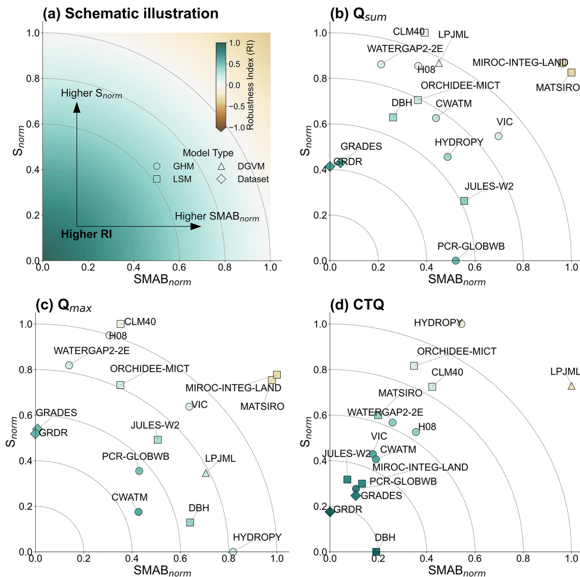
Figure 8. Assessment of model robustness in key SMR characteristics. (a) Schematic illustration. (b–d) Results for Q_{\text{sum}} , Q_{\text{max}} , and CTQ , respectively. Circles denote global hydrological models (GHMs), squares denote land surface models (LSMs), triangles denote dynamic global vegetation models (DGVMs), and diamonds denote data products. SMAB_{\text{norm}} denotes the normalized stratified mean absolute bias, and S_{\text{norm}} denotes the normalized regression slope of absolute bias. Detailed calculation procedures are provided in Sect. 2.2.4.
